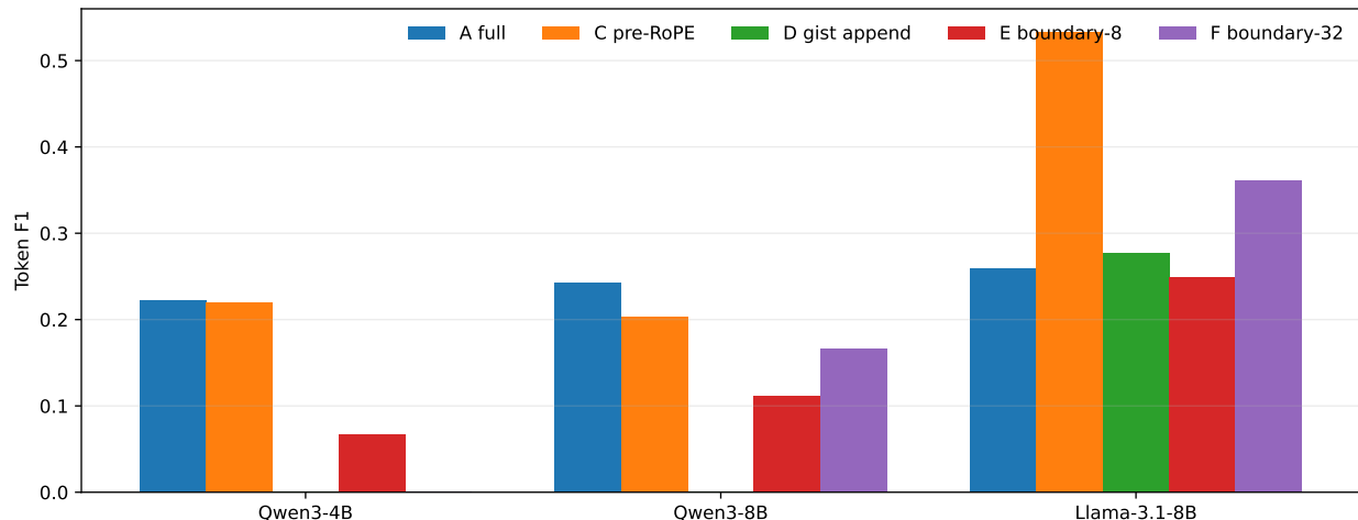
Figure 17: Token F1 in the reduced cross-model mechanism pilots. The Llama cohort shows less severe degradation, but no parameter-free composition arm improves on independent pre-RoPE K/V.
