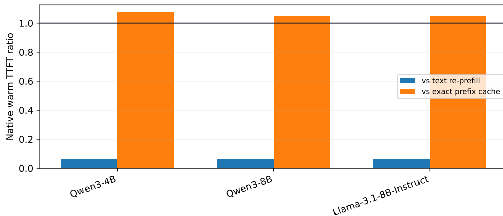
Figure 22: Warm native TTFT relative to text re-prefill and exact-prefix reuse. The horizontal line marks equal cost; lower is better.
