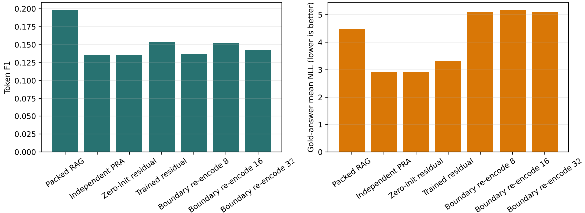
Figure 13: Task F1 and gold-answer NLL for packed RAG, independent PRA, the identity and trained residuals, and selective boundary re-encoding. Neither a smaller first-step JS nor more boundary recomputation guarantees better teacher-forced answer likelihood.
