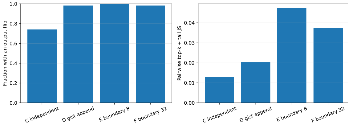
Figure 14: Post-hoc parameter-free gist K/V increases, rather than reduces, record-order sensitivity.
