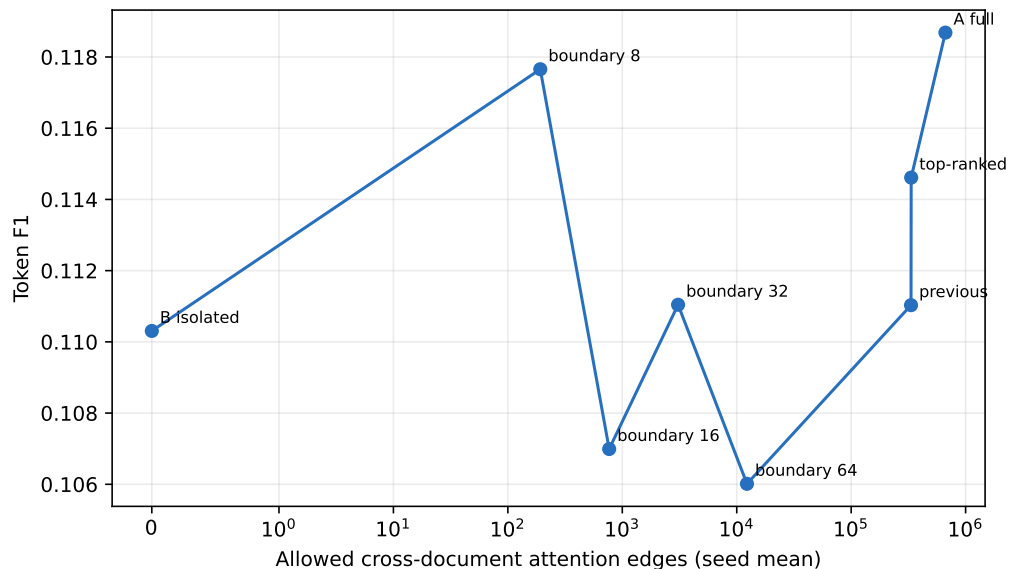
Figure 16: Token F1 against allowed document-to-document attention edges. More interaction is not monotonically better on the measured cohort.
