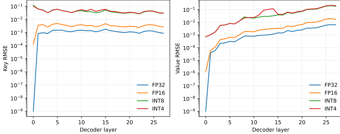
Figure 11: Layerwise independent-record B/C error under the explicit precision ladder. P2 is exactly zero at every layer and is omitted from the log axis.
