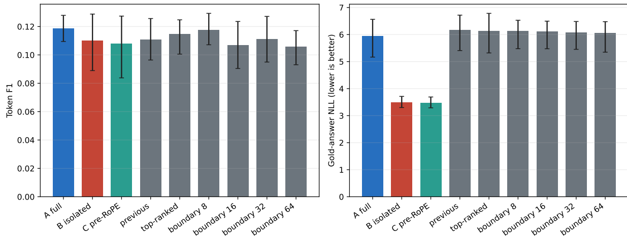
Figure 15: Task F1 and gold-answer NLL for A/B/C and the sparse mask ladder. Intervals bootstrap five seed-cohort means.
