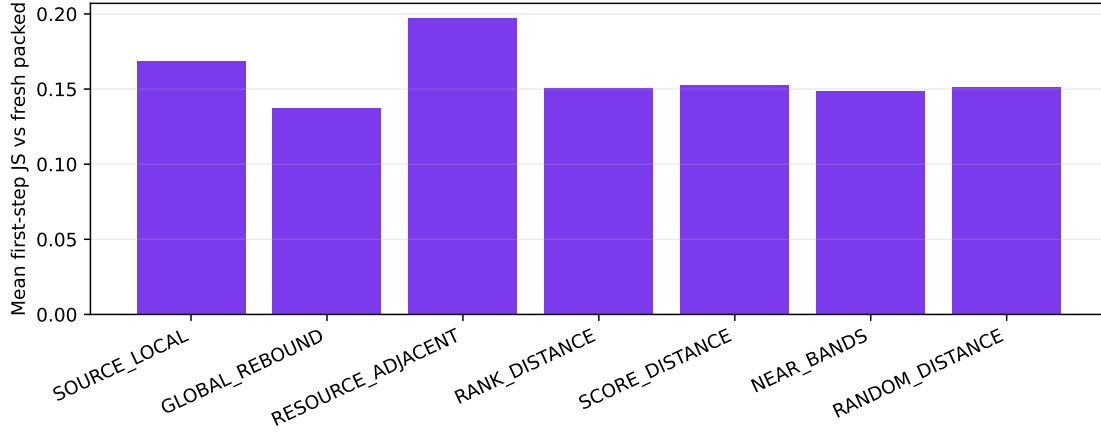
Figure 19: First-step divergence from fresh packed encoding under alternative position policies (200 order-specific comparisons per policy across five cohorts).
