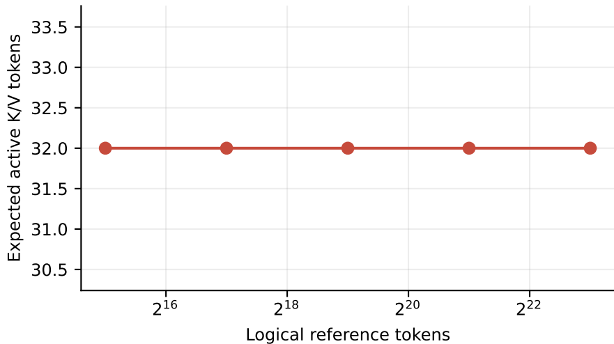
Oracle-free adaptive effort (threshold 0.06)
