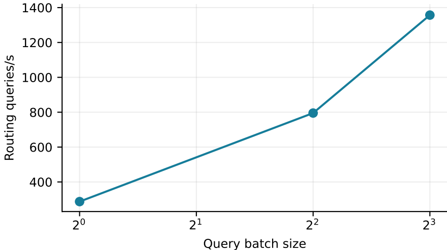
Routing throughput at 8,388,608 logical tokens
