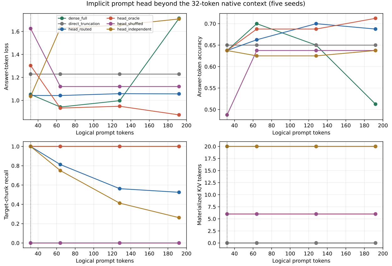
Figure 20: Quality, recall, and active memory as the implicit head grows beyond the native limit. Dense execution is shown only because this tiny source model supports 192 tokens.
