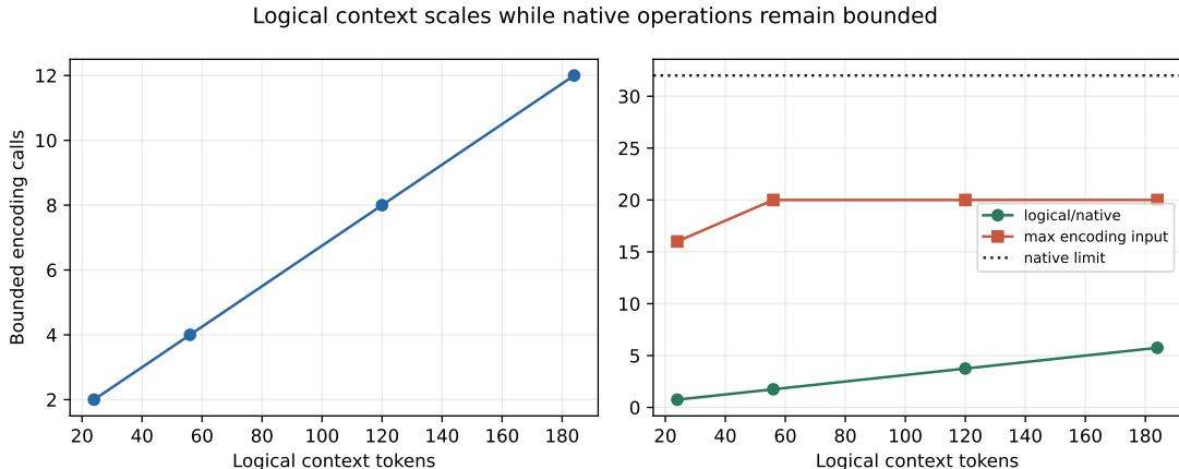
Figure 19: Model-scaled context safety. Logical head length and encoding-call count grow, while each overlap-aware base-model encoding remains below the 32-token hard limit.
