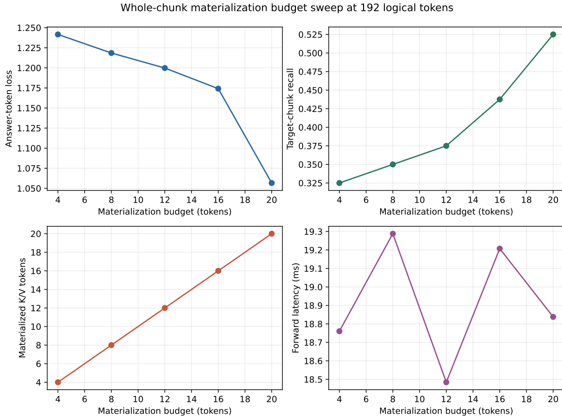
Figure 21: Quality and systems measurements under score-ordered whole-chunk admission. The sweep changes active K/V, not routing candidate count.
