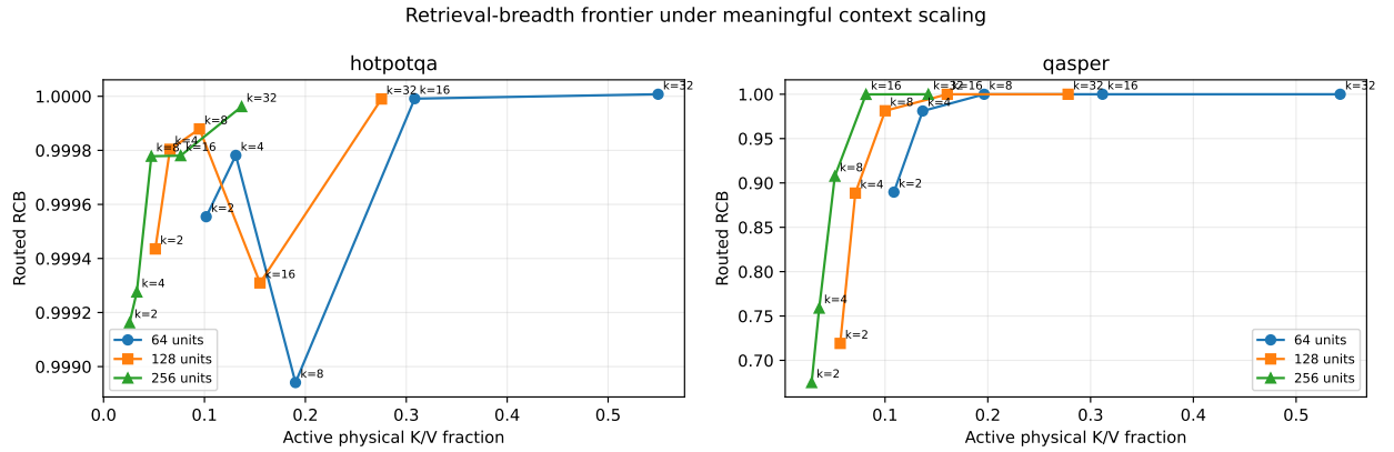
Figure 11: Tiny-backbone top- k frontier. QASPER-derived text requires increasing breadth as addressability grows: at 256 units, routed RCB rises from 0.675 at k = 2 to 0.908 at k = 8 , 1.000 at k = 16 , and 1.000 at k = 32 . HotpotQA-derived loss is nearly insensitive because the answer-bearing native state is consistently selected.
