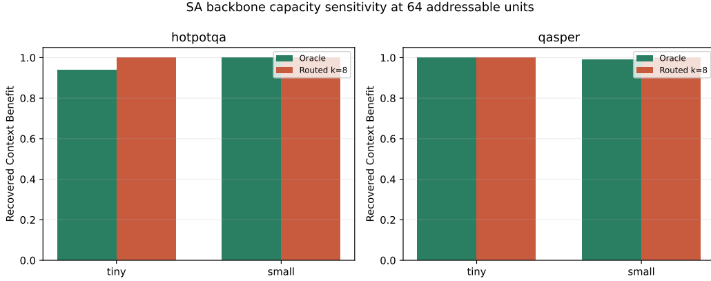
Figure 13: Backbone capacity at 64 units. The small tier improves annotated-oracle robustness and maintains routed quality, but also increases model and K/V width.
