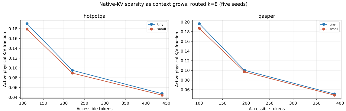
Figure 12: Physical active fraction at routed k = 8 . Retrieved token count remains nearly constant while accessible context grows, so active fraction falls approximately inversely with source size.
