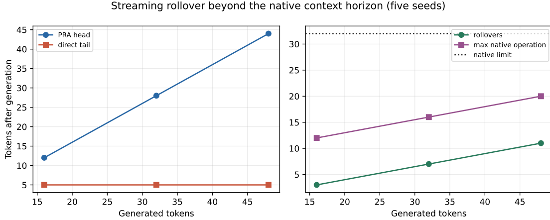
Figure 22: Streaming rollover beyond the native horizon. Direct history remains bounded; expired tokens accumulate in the routable request-local head without a native-limit violation.
