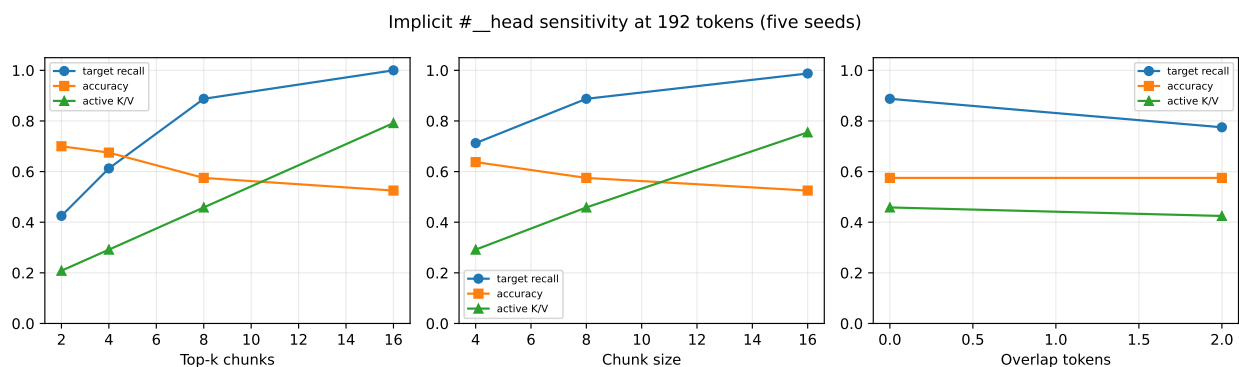
Figure 18: Implicit-head sensitivity at 192 tokens. Greater top- k improves target-chunk recall but can reduce language-model quality by admitting irrelevant K/V.
