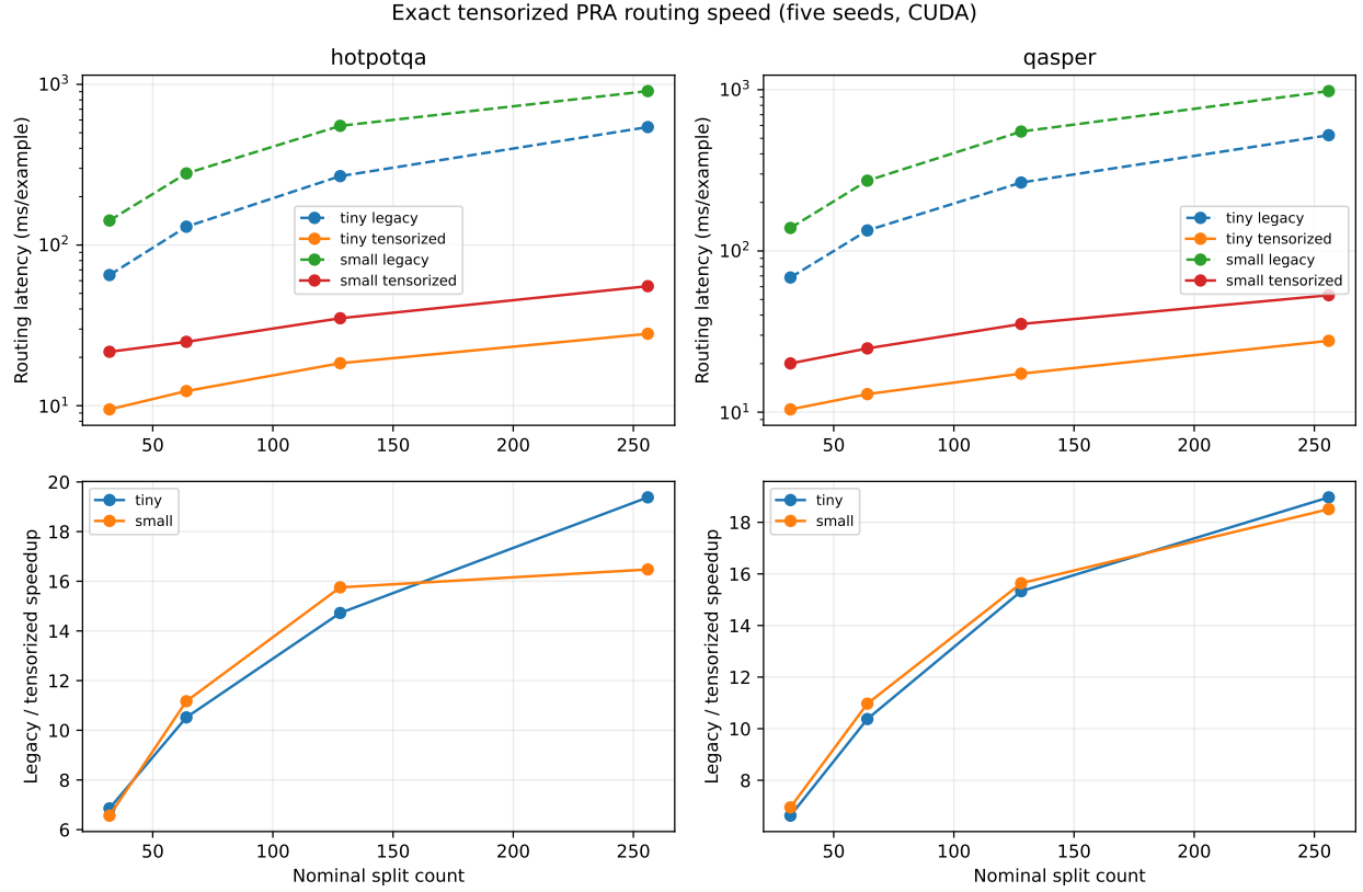
Figure 15: Exact routing latency and paired speedup at 32/64/128/256 nominal splits. The tensorized path still scores every candidate, but replaces hundreds of scalar launches and synchronizations with packed kernels; its advantage therefore grows with addressability.
