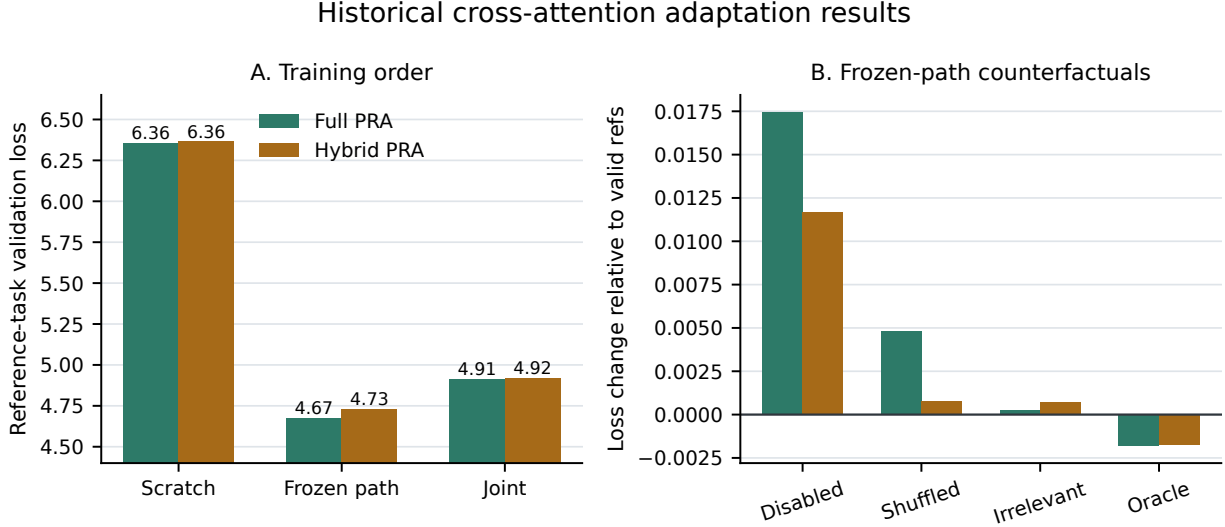
Figure 25: Historical cross-attention adaptation results. Left: frozen-path adaptation finishes substantially below scratch and direct joint tuning for both PRA placements. Right: frozen-path loss changes relative to valid references; positive values are worse. Disabling memory has a visible cost, but shuffled and irrelevant changes and oracle gains are small, so the branch effect is not evidence of content-causal retrieval.
