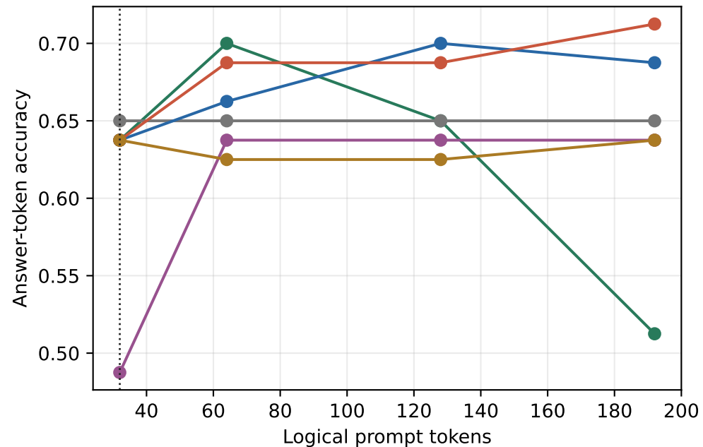
Implicit prompt head beyond the 32-token native context (five seeds)
