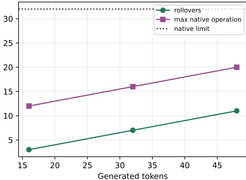
Streaming rollover beyond the native context horizon (five seeds)
