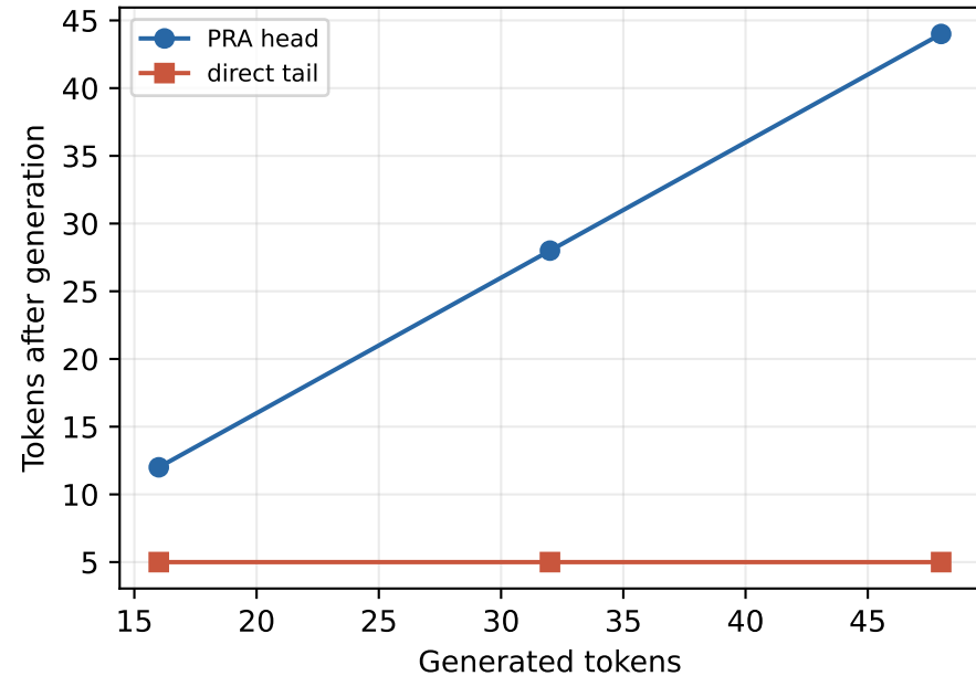
Streaming rollover beyond the native context horizon (five seeds)
