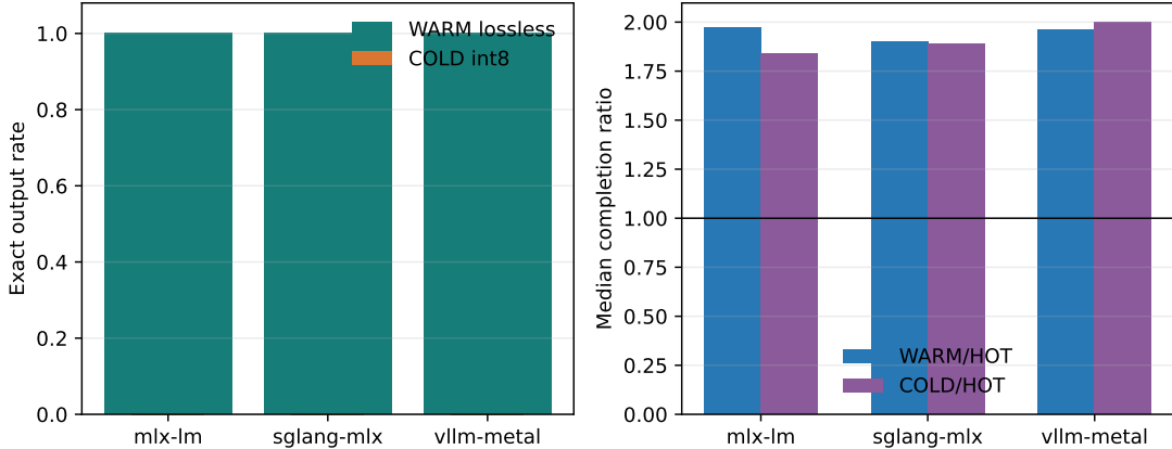
Figure 15: Lossless WARM preserves all three outputs per engine, whereas int8 COLD changes every 24-token sequence. The latency panel measures a tier hit at request time; background WARM and COLD transitions are reported separately.
