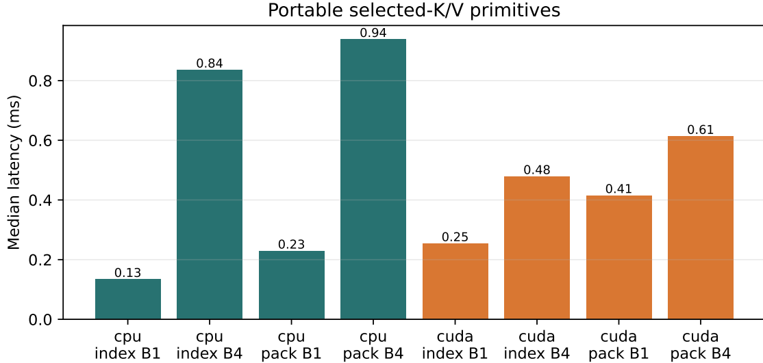
Figure 9: Portable primitive latency. This older GPU does not make small batch-one gathers faster than the CPU, but CUDA scales better at batch four.
