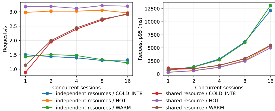
Figure 18: Shared and independent MLX resources through 16 concurrent sessions. The finite waves include promotion and serialized model queueing.
