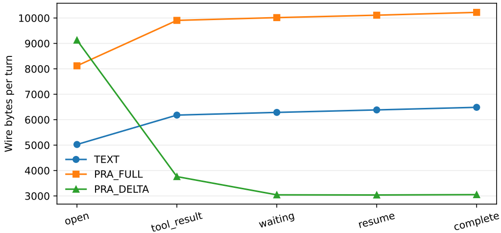
Figure 7: Per-turn JSON bytes for the five-turn task/tool workflow. PRA-FULL preserves explicit metadata but repeats all resource bodies; PRA-DELTA sends a body only for ADD or UPDATE and keeps unchanged resources logical.
