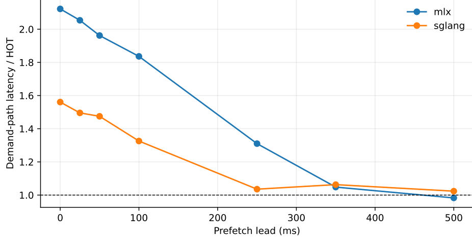
Figure 17: Scheduler-owned WARM promotion can hide request-path stall when useful lead is available. The dashed line is HOT latency.
