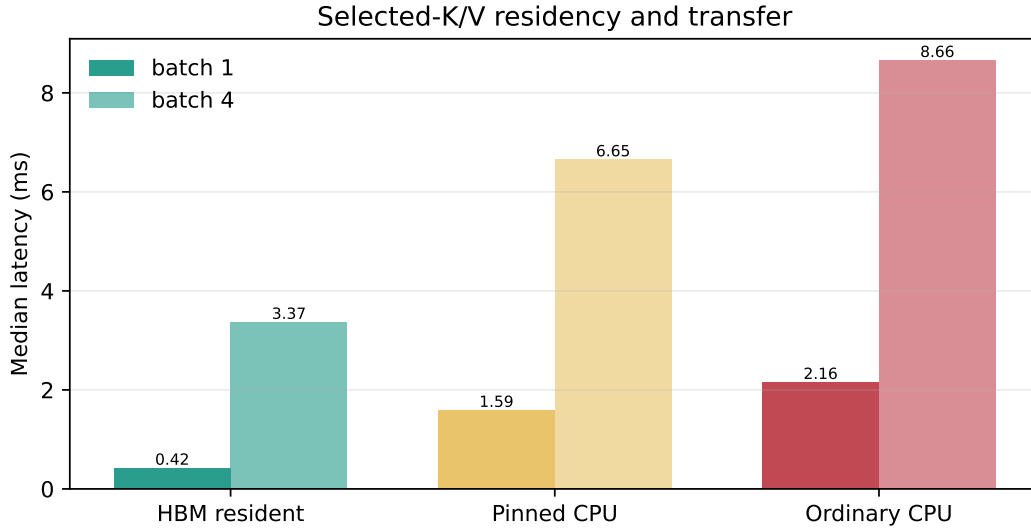
Figure 10: The same logical selection has different physical cost depending on residency. Pinned transfer helps, but does not erase the hierarchy boundary.
