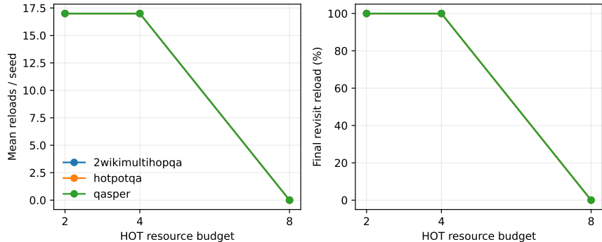
Figure 19: Sustained pressure exposes a working-set threshold rather than a quality effect: once all eight resources fit, reloads disappear.
