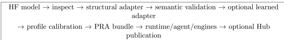
Figure 23: The model-onboarding path. Each arrow is a separately inspectable service boundary rather than an implicit side effect of one CLI callback.
