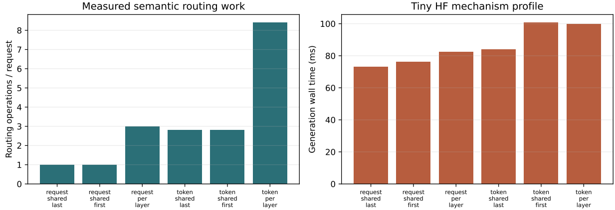
Figure 8: Five-seed tiny-HF mechanism profile. Routing operations validate the execution contract; wall time is host- and model-specific and is not a serving speed claim.
