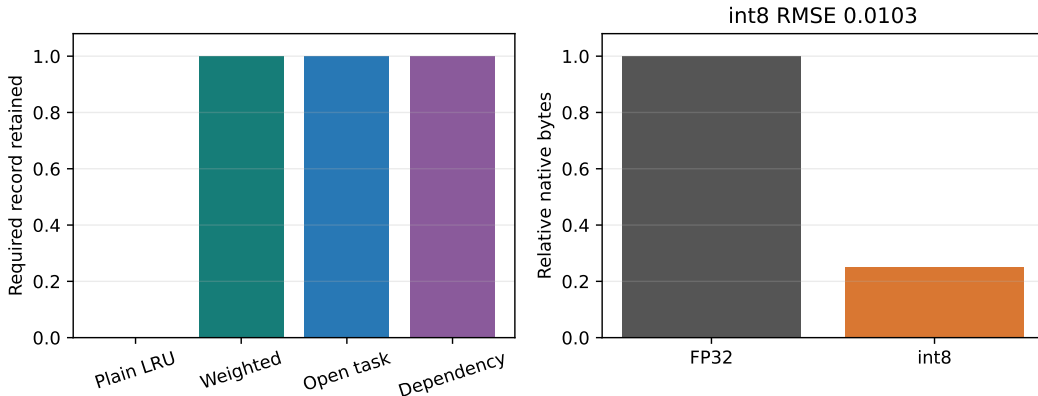
Figure 14: Engine-neutral retention controls and generic symmetric-int8 byte transport. The int8 result is a codec diagnostic; model-specific quality and active-attention bytes remain separate gates.
