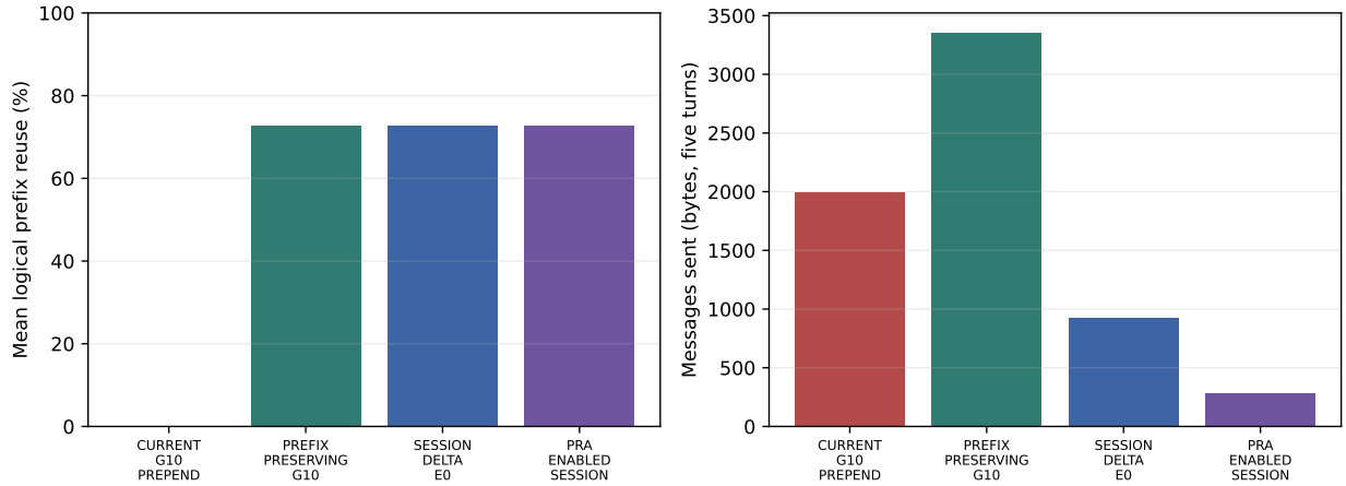
Figure 6: Five-turn deterministic gateway profile. The left panel reports logical reuse of the exact prior serialized message prefix after turn one; the right reports message bytes sent. Resource bytes are reported separately in Table 7.
