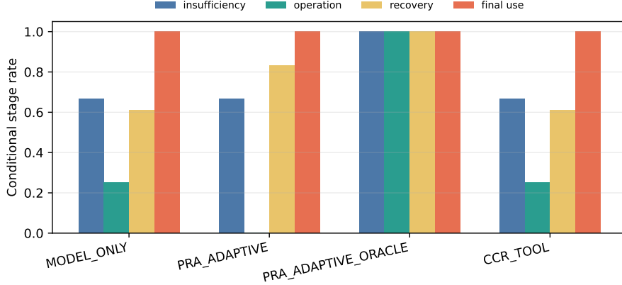
Figure 5: The adaptive gap decomposes into insufficiency detection, operation choice, and final evidence use. Oracle headroom does not imply that a larger controller is automatically cost-effective.
