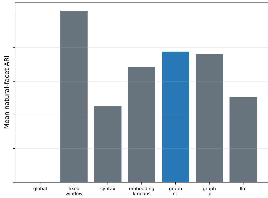
SmolLM2-135M
