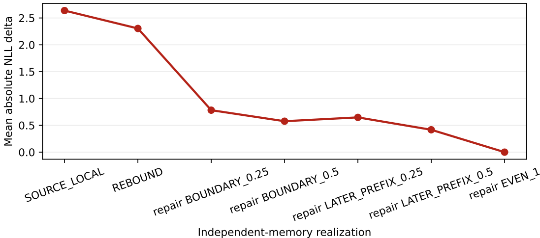
Figure 16: Position rebinding and deterministic contextual repair reduce the composition error, but all five cohorts reach exact parity only at full repair. Repair timings are diagnostic because fresh packed states were computed first.
