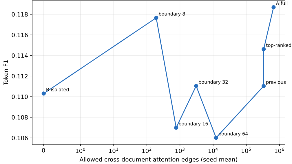
Figure 15: Token F1 against allowed document-to-document attention edges. More interaction is not monotonically better on the measured cohort.
