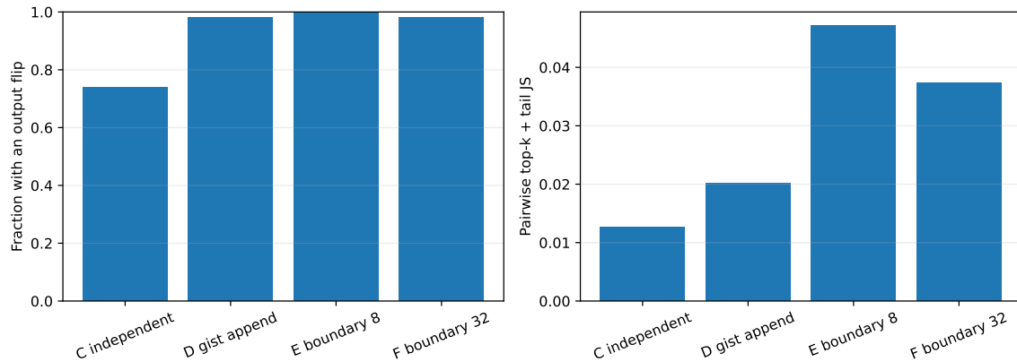
Figure 13: Post-hoc parameter-free gist K/V increases, rather than reduces, record-order sensitivity.
