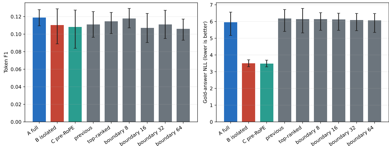
Figure 14: Task F1 and gold-answer NLL for A/B/C and the sparse mask ladder. Intervals bootstrap five seed-cohort means.
