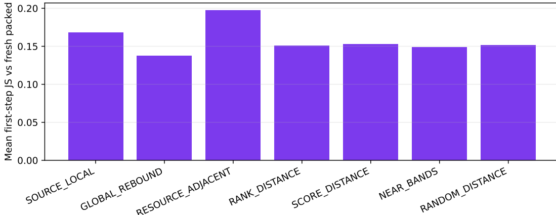
Figure 17: First-step divergence from fresh packed encoding under alternative position policies (200 order-specific comparisons per policy across five cohorts).
