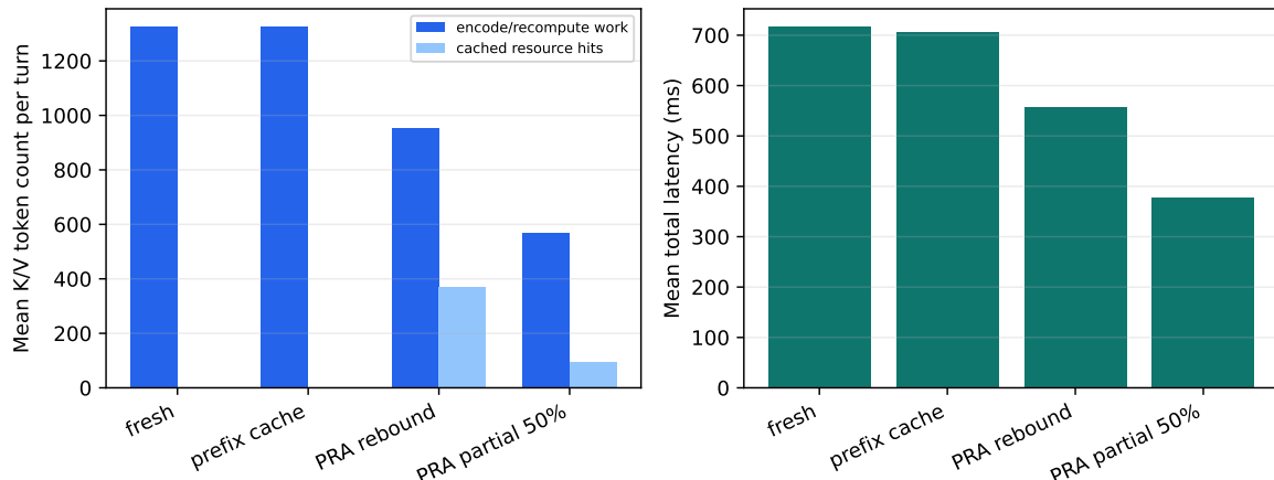
Figure 19: Five-seed mean per-turn K/V accounting and measured latency under changing selections. Encoding/recomputation and cache hits are shown as separate bars rather than as an active-context stack. Diagnostic repair is omitted because copying precomputed fresh states is not a deployable timing.
