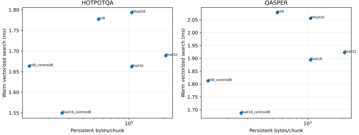
Figure 8: Warm vectorized search versus persistent routing-index bytes. Quantization changes residency far more than latency on this small, old GPU.
