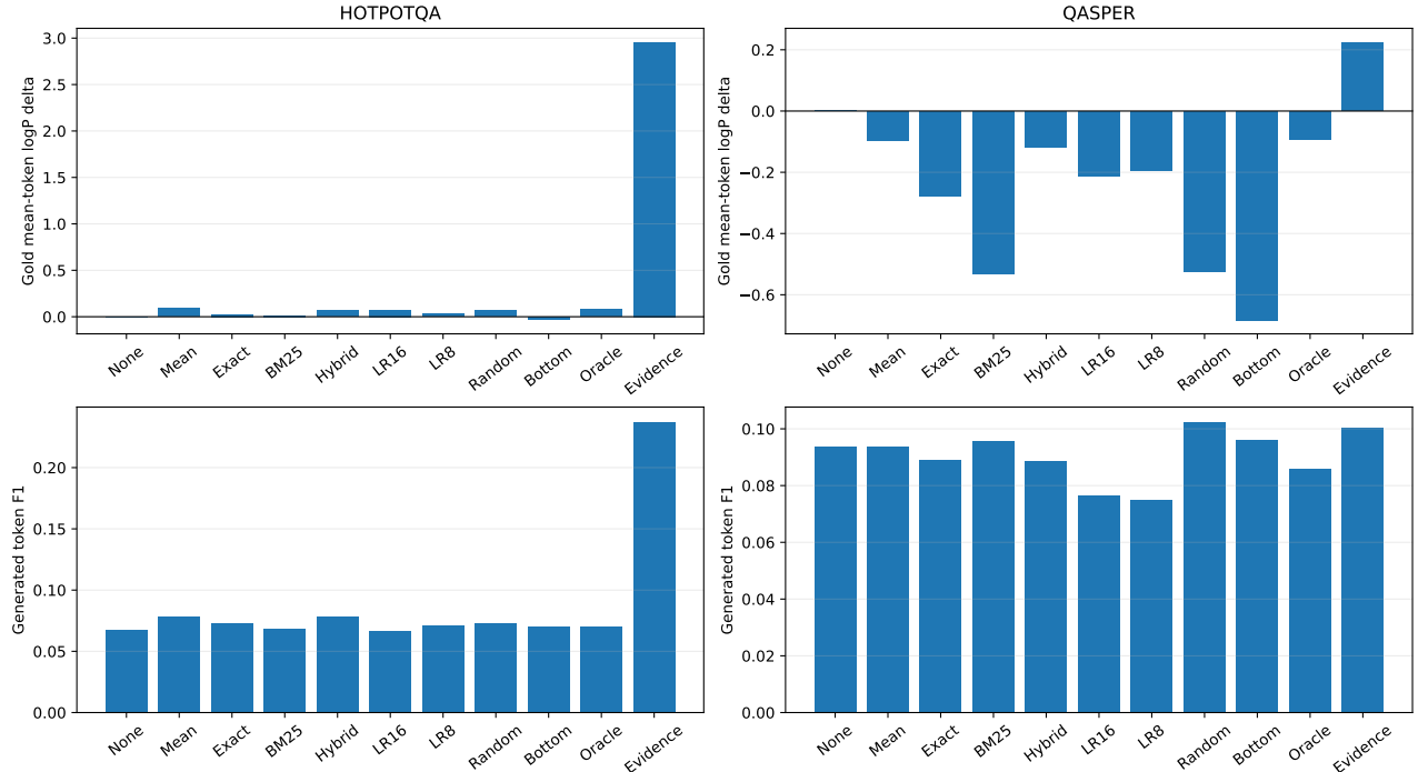
Figure 7: Native-K/V generation and causal controls. Routing quality and memory integration are distinct bottlenecks.
