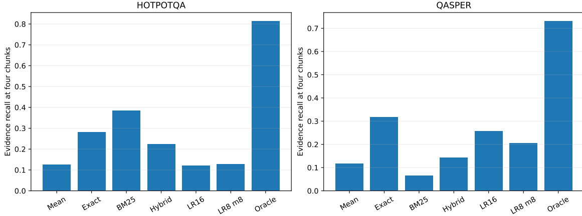
Figure 6: Fresh-cohort routing confirmation. The rank-16 gain transfers within QASPER, while Hotpot remains lexical.
