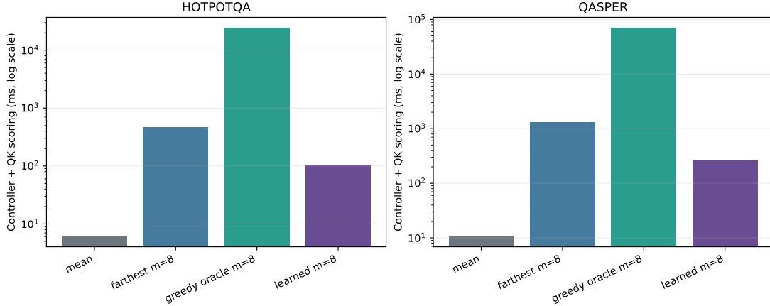
Figure 10: Controller construction plus QK scoring on a log scale. The oracle is a feasibility instrument, not a serving method.
