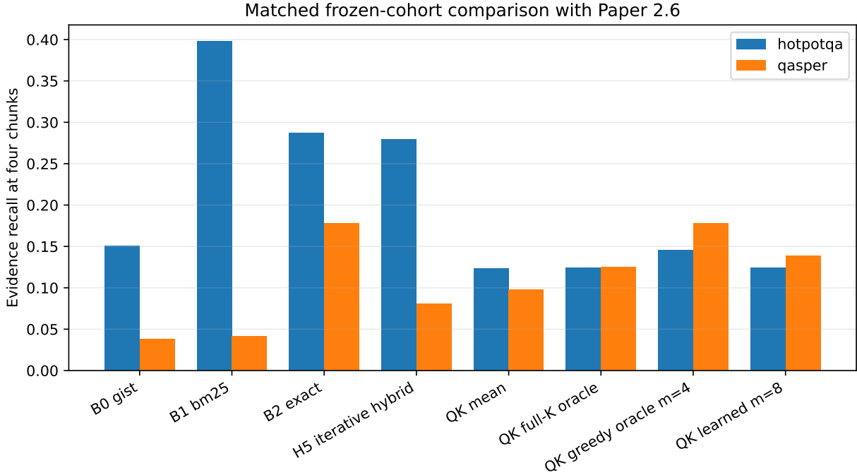
Figure 9: Matched Paper 2.6 comparison. Full-K and greedy rows are non-deployable upper bounds. Learned QK is competitive on QASPER but not Hotpot.
