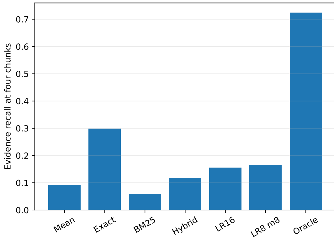
QASPER
