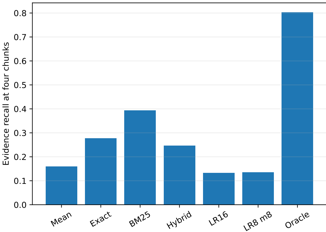
HOTPOTQA
