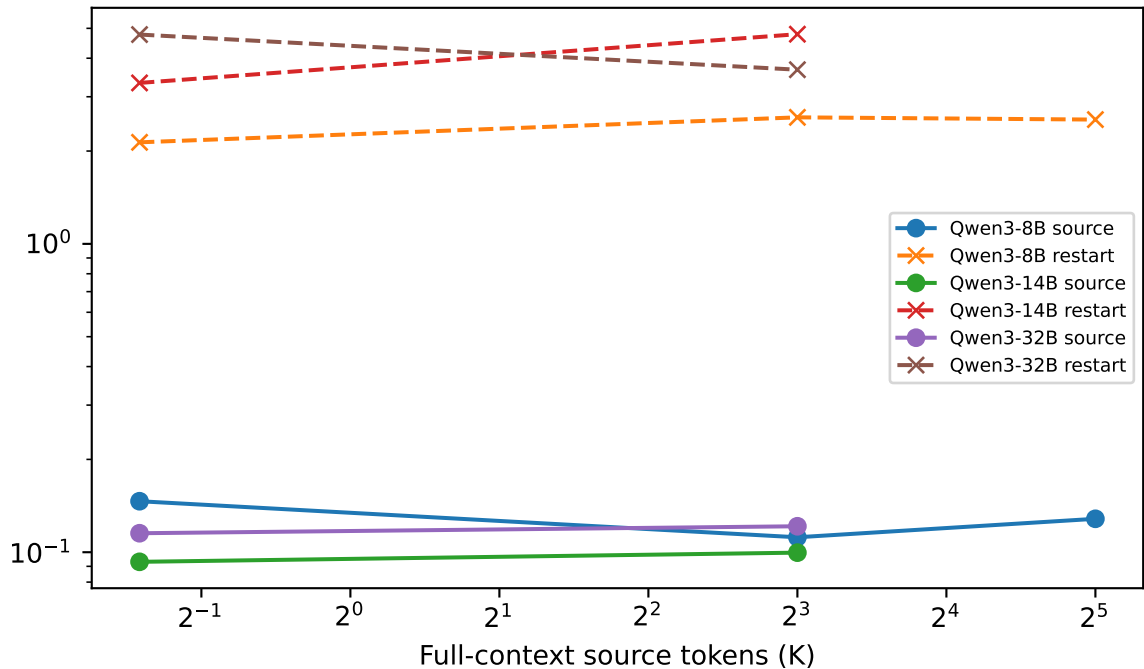
First-logit RMSE vs ordinary prefix
