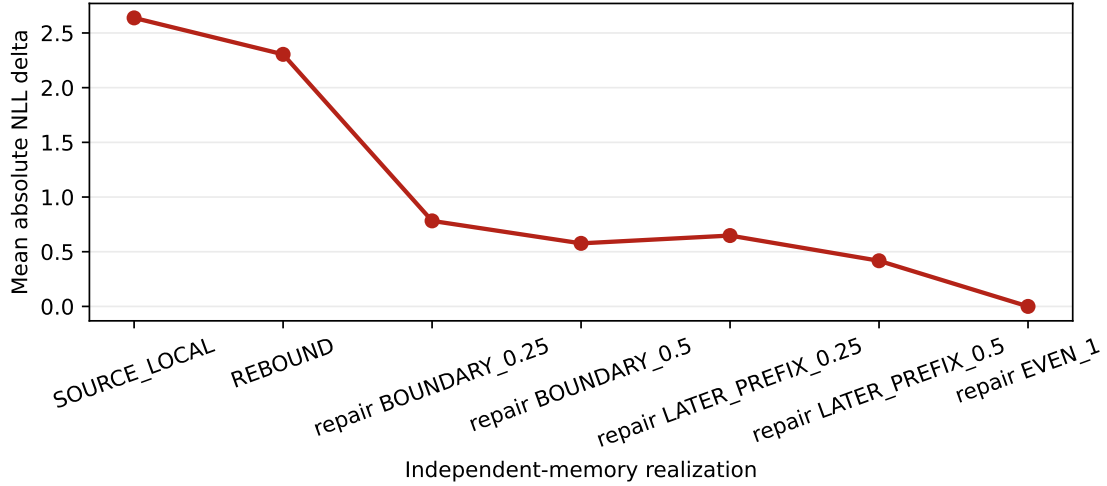
Figure 14: Position rebinding and deterministic contextual repair reduce the composition error, but all five cohorts reach exact parity only at full repair. Repair timings are diagnostic because fresh packed states were computed first.
