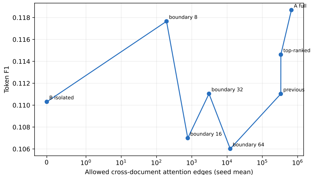
Figure 13: Token F1 against allowed document-to-document attention edges. More interaction is not monotonically better on the measured cohort.
