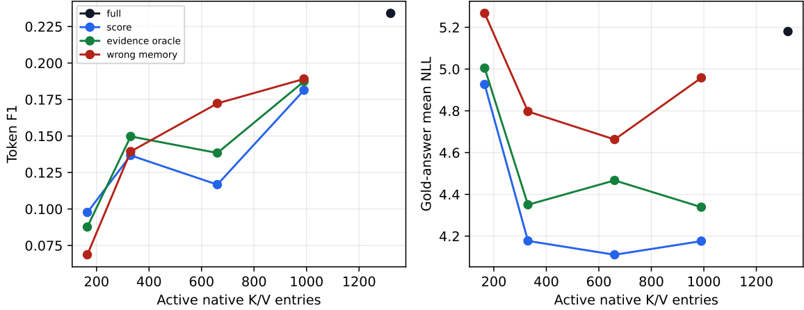
Figure 16: Quality and gold-answer NLL against active native K/V. The different metrics need not rank small-sample generations identically.
