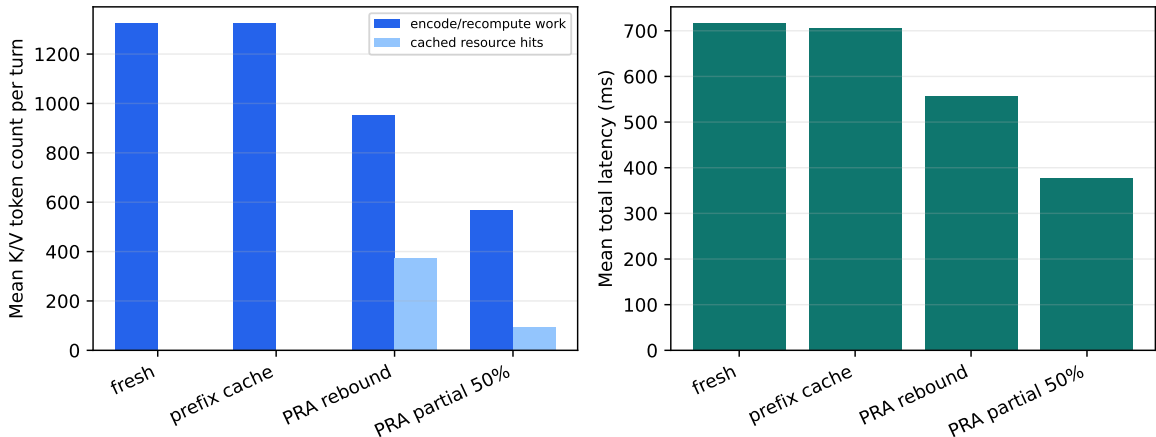
Figure 17: Five-seed mean per-turn K/V accounting and measured latency under changing selections. Encoding/recomputation and cache hits are shown as separate bars rather than as an active-context stack. Diagnostic repair is omitted because copying precomputed fresh states is not a deployable timing.
