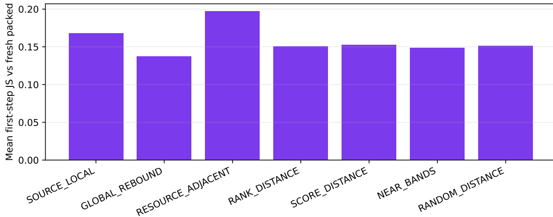
Figure 15: First-step divergence from fresh packed encoding under alternative position policies (200 order-specific comparisons per policy across five cohorts).
