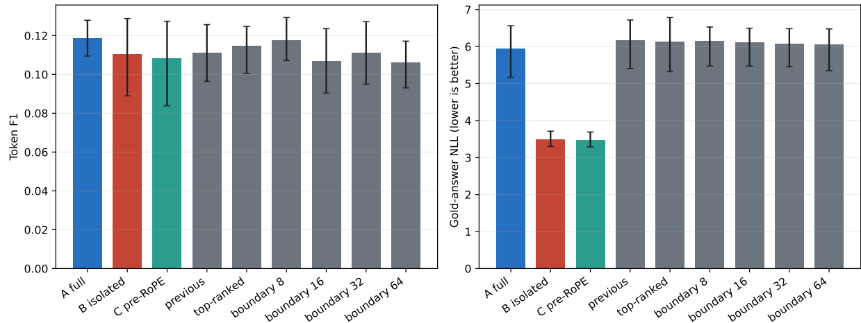
Figure 12: Task F1 and gold-answer NLL for A/B/C and the sparse mask ladder. Intervals bootstrap five seed-cohort means.
