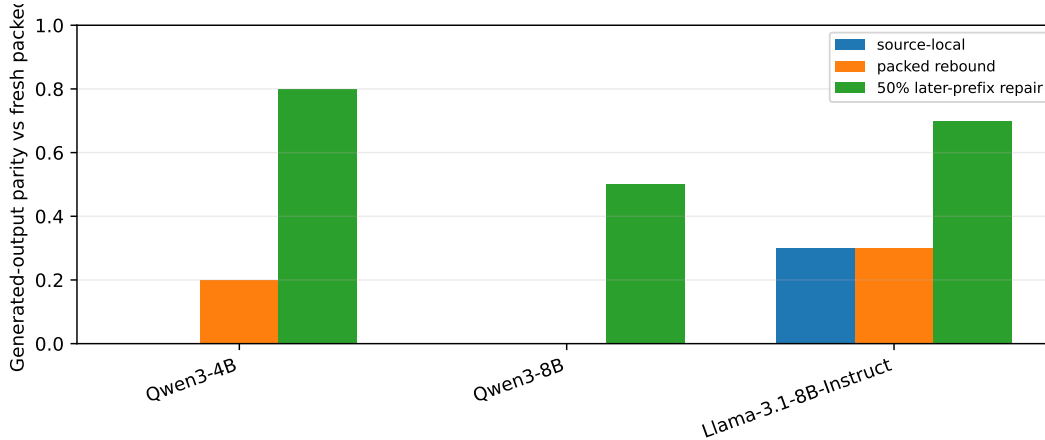
Figure 19: Independent-composition output parity on the reduced scale cohort. Full repair, omitted for scale, is 1.0 for all three models.
