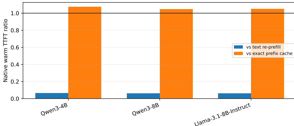
Figure 18: Warm native TTFT relative to text re-prefill and exact-prefix reuse. The horizontal line marks equal cost; lower is better.
