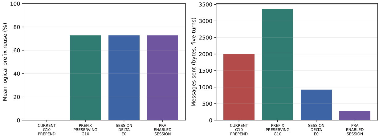
Figure 7: Five-turn deterministic gateway profile. The left panel reports logical reuse of the exact prior serialized message prefix after turn one; the right reports message bytes sent. Resource bytes are reported separately in Table 9.
