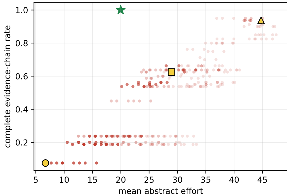
hotpotqa
