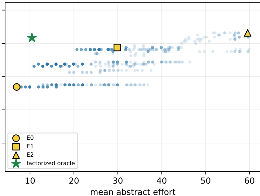
qasper
