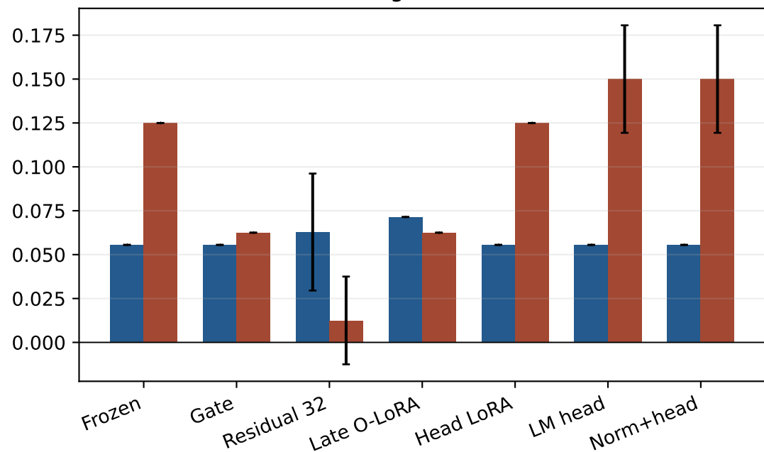
No-PRA WikiText-2 loss change
