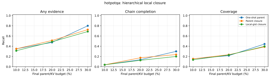
Figure 18: Gate-2 HotpotQA curves under matched final parent budgets. Local routing exposes stronger subchunk edges but does not improve evidence-group chain completion.
