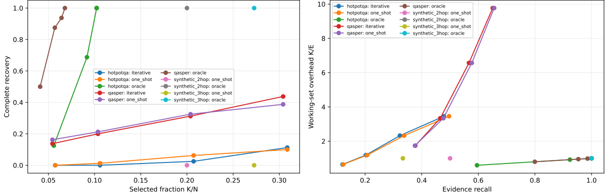
Figure 16: Per-budget complete recovery (left) and evidence-normalized working-set overhead (right). Dataset-specific rows and evidence-count strata are exported in the accompanying CSV artifacts.
