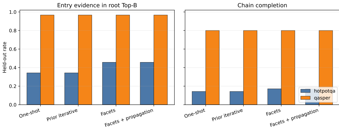
Figure 26: Entry discovery and downstream chain completion for the four confirmation methods. Facets improve Hotpot entry and chain metrics while preserving QASPER; propagation does not add chain completion beyond the new root at this budget.
