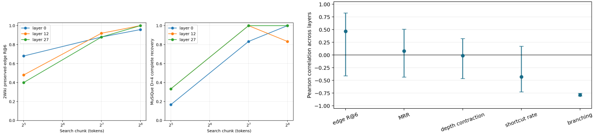
Figure 15: Pretrained layer-by-granularity topology and matched contextualization correlations. No single late or highly contextual layer dominates every graph scale.
