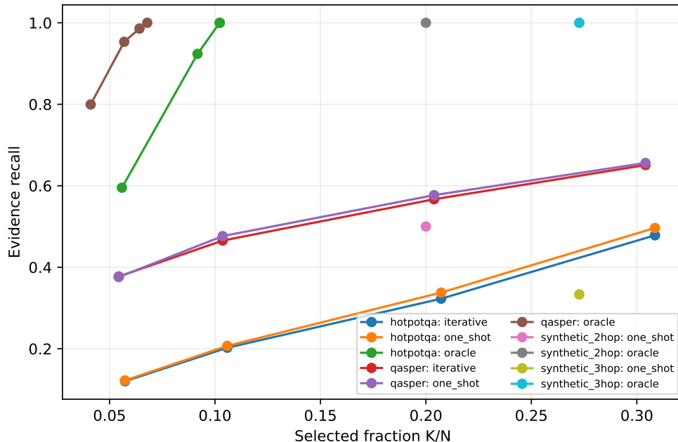
Figure 12: Evidence recall against actual selected fraction across measured budgets. Only the oracle crosses the predeclared .80/.90/.95 targets; no \phi_{80} , \phi_{90} , or \phi_{95} is extrapolated for executable routes.
