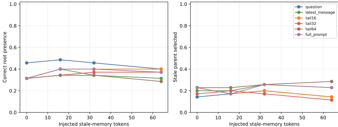
Figure 28: Held-out Hotpot response to injected stale-memory text. Left: current root entry. Right: selection of the explicitly non-oracle stale parent. The validation-frozen latest-message boundary is bounded and cheaper, but stale-context resistance remains mixed on this sample.
