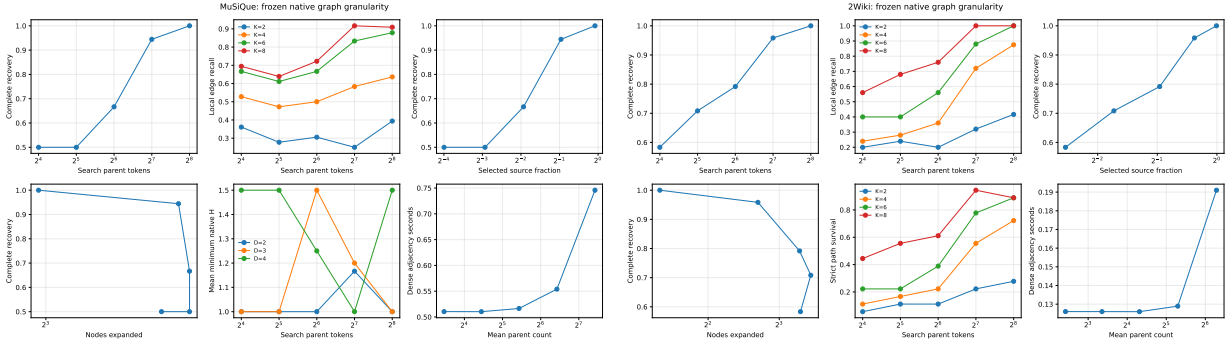
Figure 36: Frozen native graph granularity. Finer nodes reduce selected payload and increase evidence density, but direct edge and complete recovery deteriorate. Dense exact adjacency remains the cold-cost bottleneck; search itself is milliseconds.
