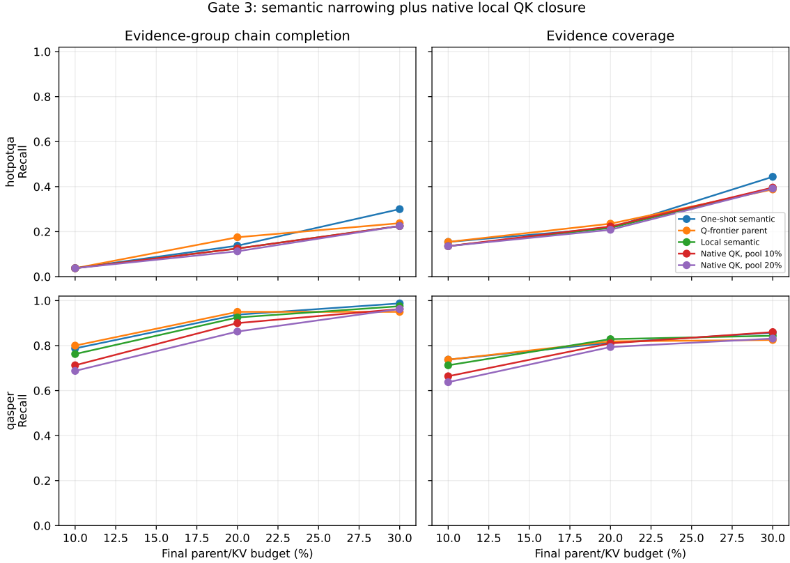
Figure 19: Gate-3 chain completion and evidence coverage across final budgets. Primary native-QK propagation does not dominate local semantic or one-shot routing; the larger candidate pool is usually worse, especially on the direct-retrieval QASPER control.
