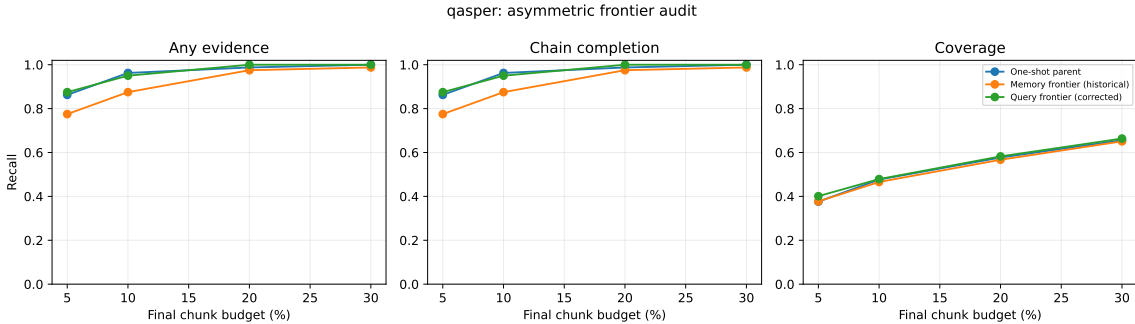
Figure 17: Gate-1 QASPER curves. Respecting the asymmetric projection contract recovers most of the historical closure loss, but one-shot remains the sparse-retrieval reference.
