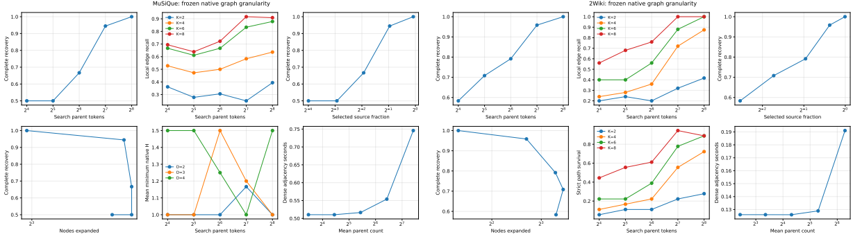
Figure 14: Granularity changes both conceptual payload and complete evidence recovery. Fine memory is sparse but topologically fragile; coarse memory is reachable but distractor rich.
