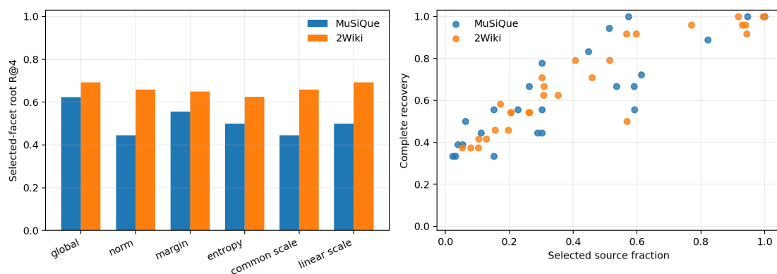
Figure 13: Executable root selectors remain below the oracle query-view ceiling; high complete recovery also requires broad conceptual activation.
