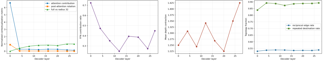
Figure 38: Measured contextualization and topology. Accumulated dependence on context grows while local attention contribution generally shrinks. Depth contraction and neighbor reuse vary, but the graph does not become uniformly more faithful.
