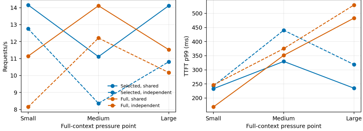
Figure 3: Peak-load throughput and TTFT tail as full visible context grows. Selected context remains fixed; solid lines share one resource and dashed lines use independent resource identities.
