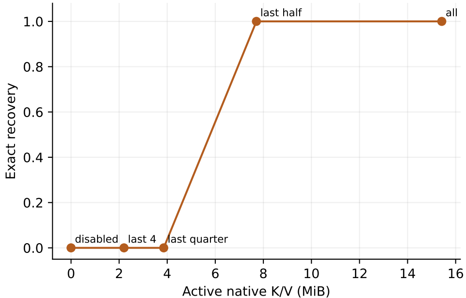
MLX consumer-layer frontier
