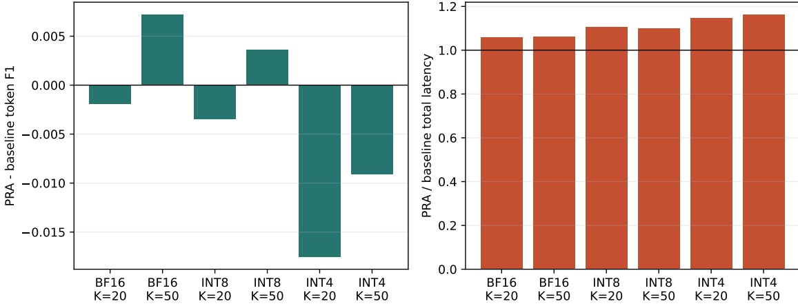
Figure 31: Quality and latency changes for the matched BF16, INT8, and INT4 deployed pipelines. The small one-seed cohort is directional evidence, not a precision invariance claim.
