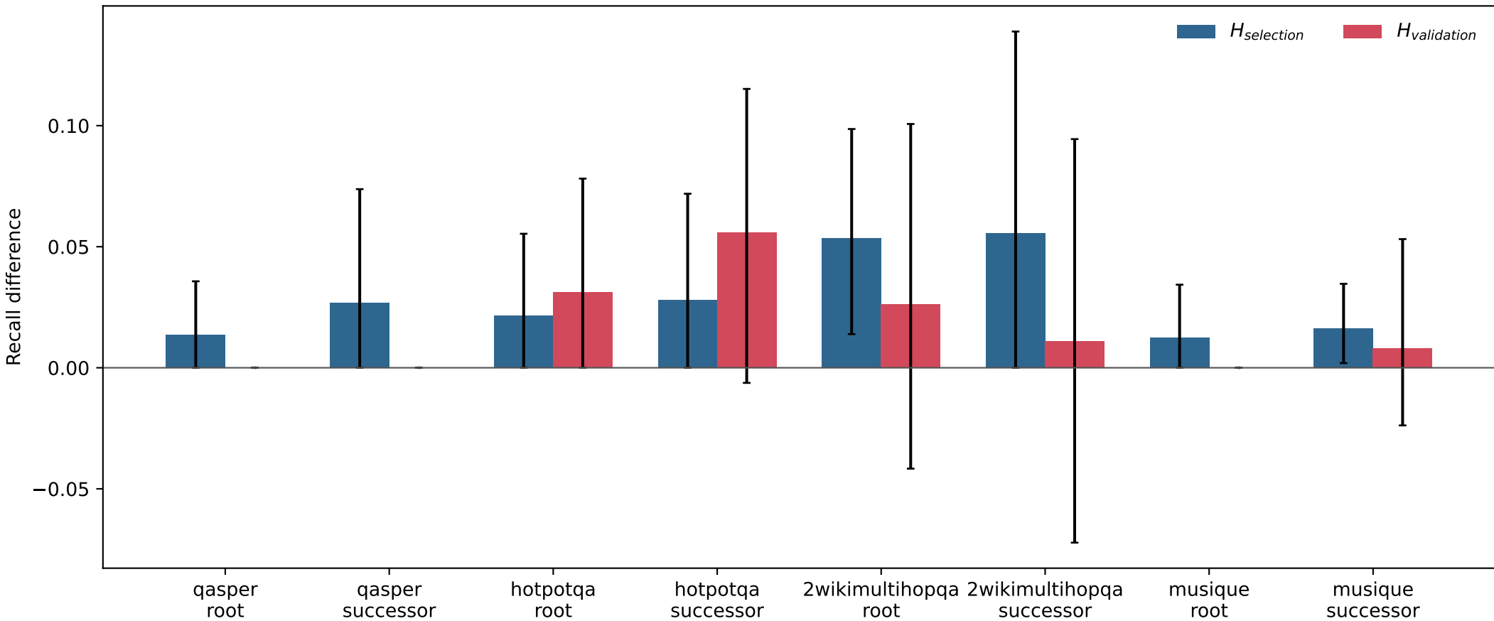
Adaptive opportunity and validation-selection instability
