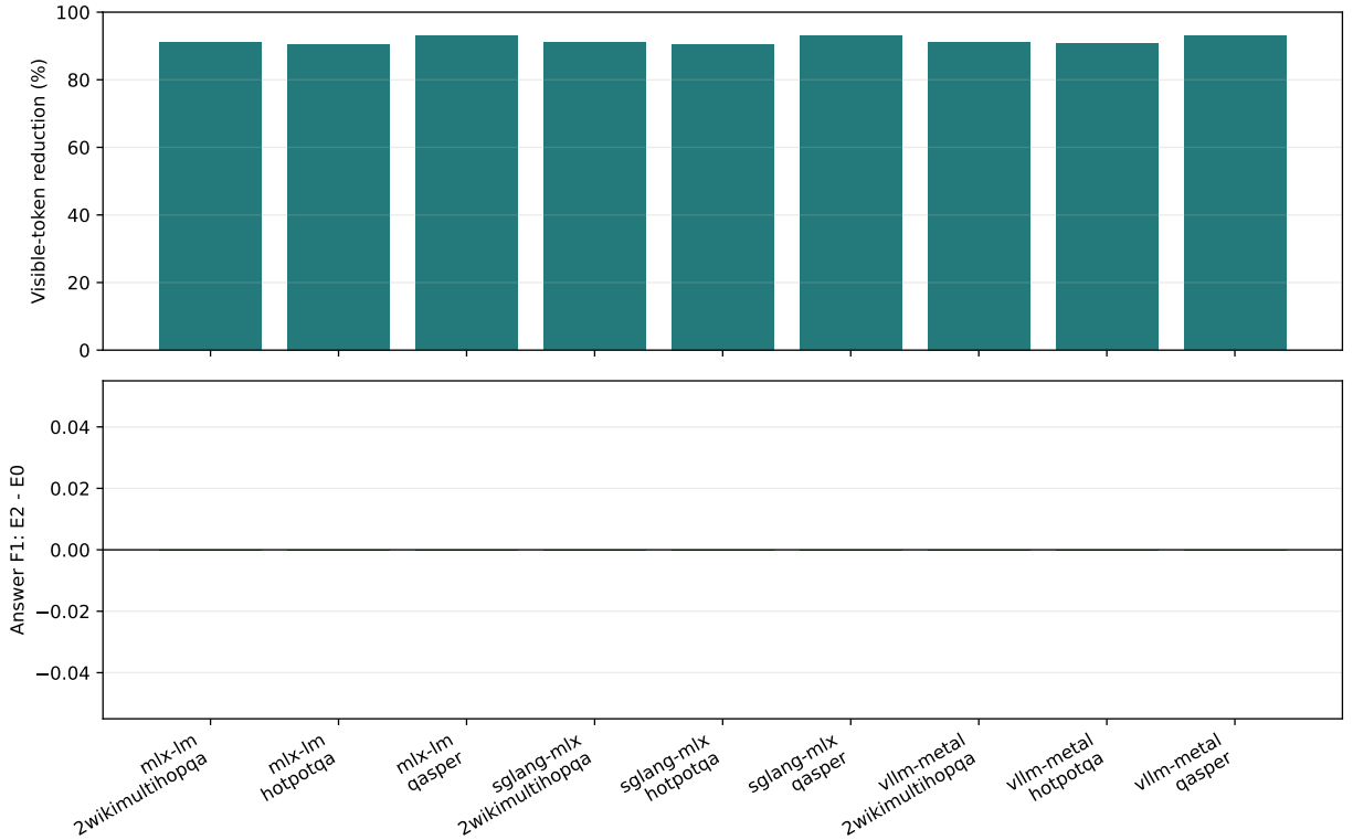
Figure 18: Holding routed evidence fixed separates visible-token reduction from semantic preservation. After restoring E0 through APC and capturing E2 from the same source prefill, all three engines retain every paired output and F1.
