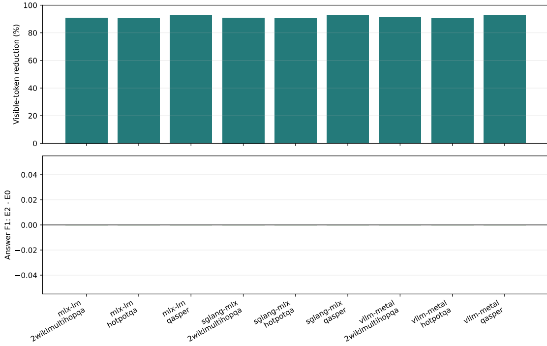
Figure 20: Expanded frozen-selection quality and visible-token accounting. Every engine preserves every paired output; confidence reflects finite sample size.
