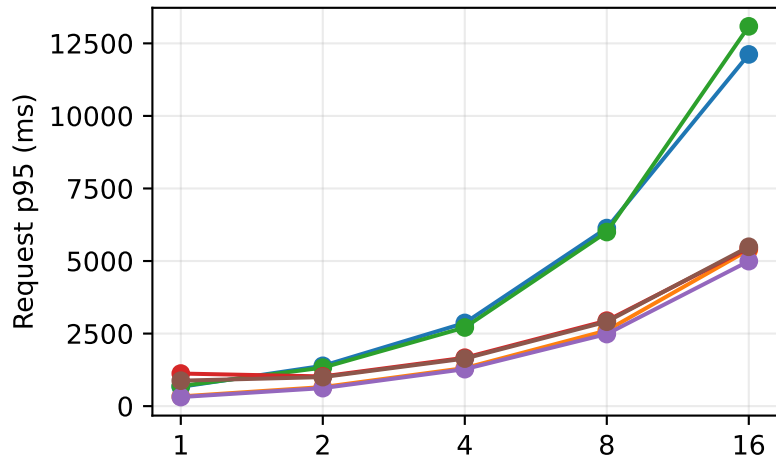
Concurrent sessions shared resource / COLD_INT8 shared resource / HOT shared resource / WARM shared resource / WARM
