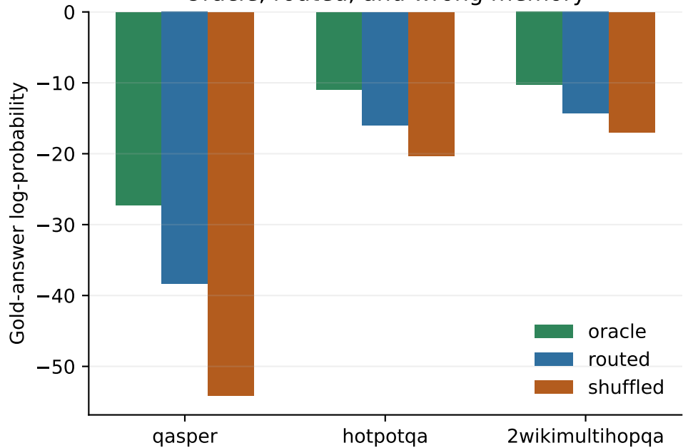
Oracle, routed, and wrong memory
