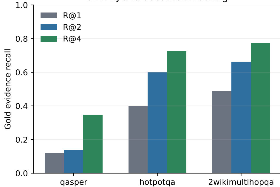
SDK hybrid document routing
