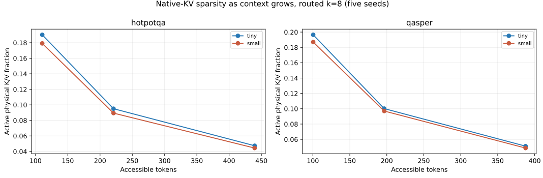
Figure 4: Fixed k = 8 keeps physical selected K/V nearly flat as candidate memory grows. The resulting active fraction falls to 4.4–4.9% at split 256 (255 source units).
