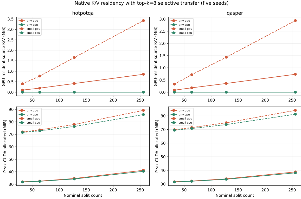
Figure 8: CPU residency removes the full inactive source cache from GPU while preserving the sparse selected payload. At split 256 the measured saving is .734–3.420 MiB; total peak CUDA allocation falls less because model parameters and other tensors remain resident.
