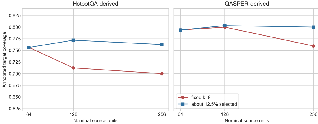
Figure 5: Fixed- k decline partly reflects increasing sparsity, not intrinsic routing collapse. Holding selection near 12.5% yields stable annotated target coverage through the measured split-256 scale.
