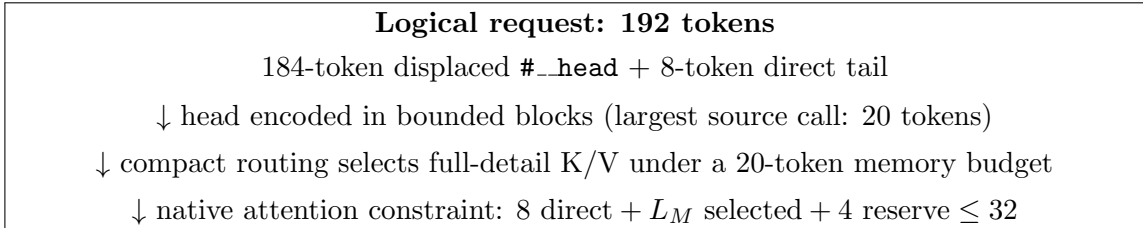
Figure 6: A 192-token logical request executes with source inputs no longer than 20 tokens and a combined attention K/V axis no longer than 28 under the configured 32-token limit. Logical history, displaced head, direct tail, retained memory, and combined K/V length are distinct quantities; the four-token reserve is unused capacity.
