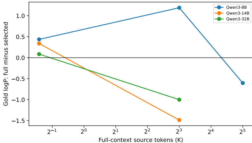
Figure 3: Full-minus-selected answer log-probability changes sign across model size and context. Selection bounds active evidence; it does not guarantee a quality advantage on every question.
