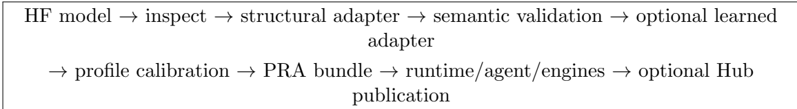
Figure 12: The model-onboarding path. Each arrow is a separately inspectable service boundary rather than an implicit side effect of one CLI callback.
