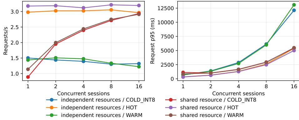
Figure 22: Shared and independent MLX resources through 16 concurrent sessions. The finite waves include promotion and serialized model queueing.
