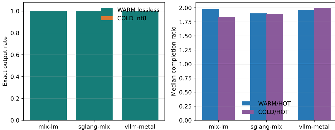
Figure 19: Lossless WARM preserves all three outputs per engine, whereas int8 COLD changes every 24-token sequence. The latency panel measures a tier hit at request time; background WARM and COLD transitions are reported separately.
