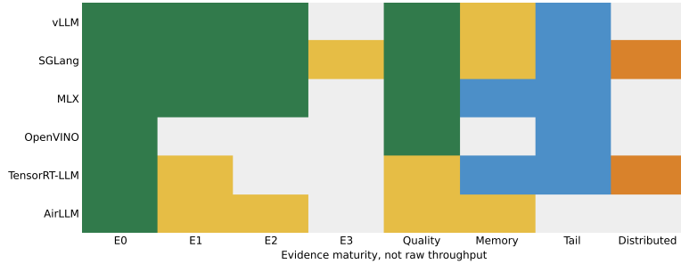
Figure 24: Cross-engine evidence maturity. Darker cells indicate stronger evidence; candidate mechanisms do not automatically promote validated level.
