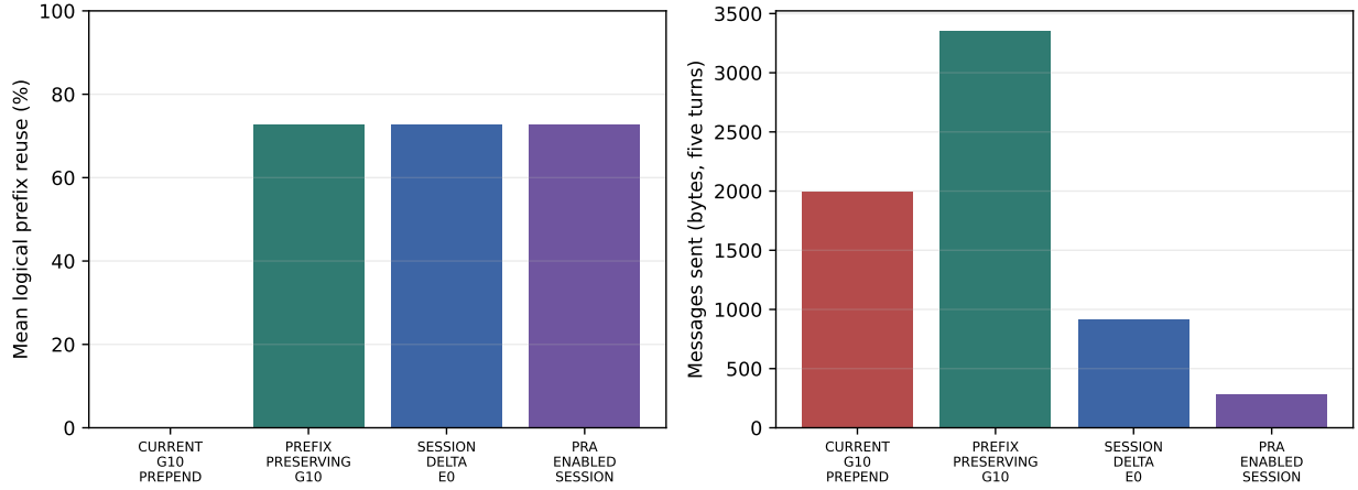
Figure 8: Five-turn deterministic gateway profile. The left panel reports logical reuse of the exact prior serialized message prefix after turn one; the right reports message bytes sent. Resource bytes are reported separately in Table 11.
