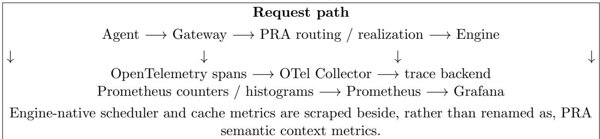
Figure 31: The observability boundary. W3C context joins request causality, while Prometheus and Grafana correlate semantic context decisions with engine-native serving behavior.
