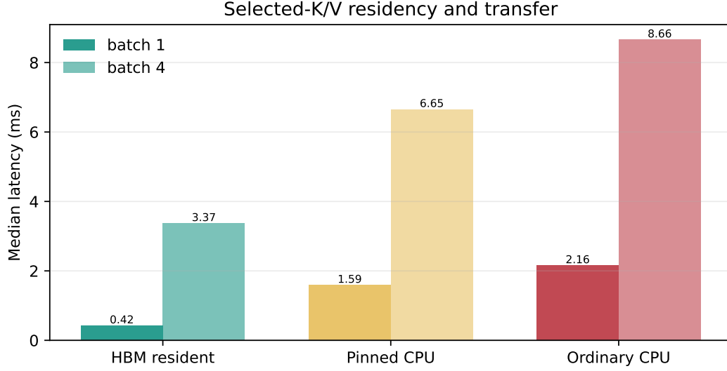
Figure 13: The same logical selection has different physical cost depending on residency. Pinned transfer helps, but does not erase the hierarchy boundary.
