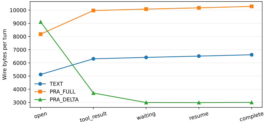
Figure 9: Per-turn JSON bytes for the five-turn task/tool workflow. PRA-FULL preserves explicit metadata but repeats all resource bodies; PRA-DELTA sends a body only for ADD or UPDATE and keeps unchanged resources logical.
