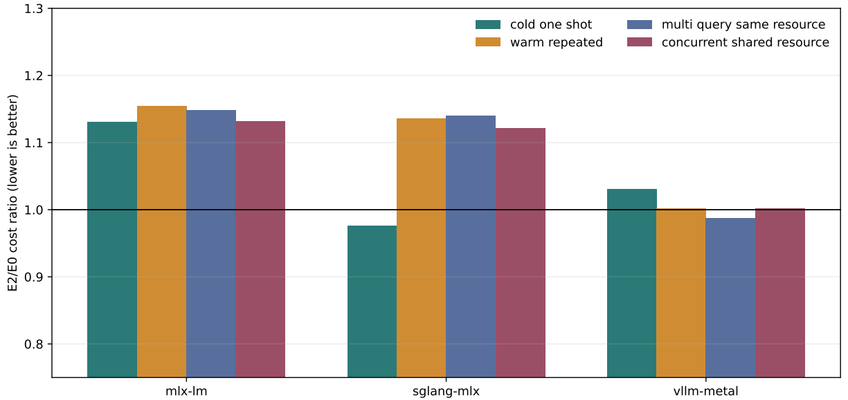
Figure 13: Representation economics after freezing retrieval. Ratios below one favor native E2. The current SGLang path wins only cold ingestion-inclusive cost; vLLM is near parity; MLX and SGLang still pay unfused decode overhead in reused and concurrent regimes.
