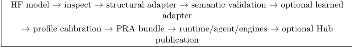
Figure 14: The model-onboarding path. Each arrow is a separately inspectable service boundary rather than an implicit side effect of one CLI callback.
