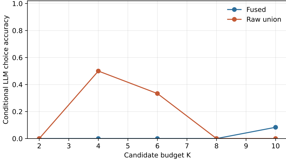
Figure 31: Conditional model choice across candidate budgets. A resolver gain becomes operational only when the model can distinguish target from admitted distractors.
