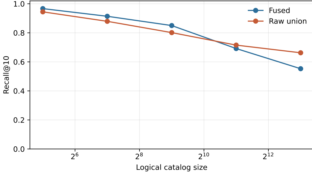
Figure 30: Five-seed large-catalog Recall@10. Union increasingly helps candidate generation as the logical catalog grows, before any candidate is shown to the generation model.
