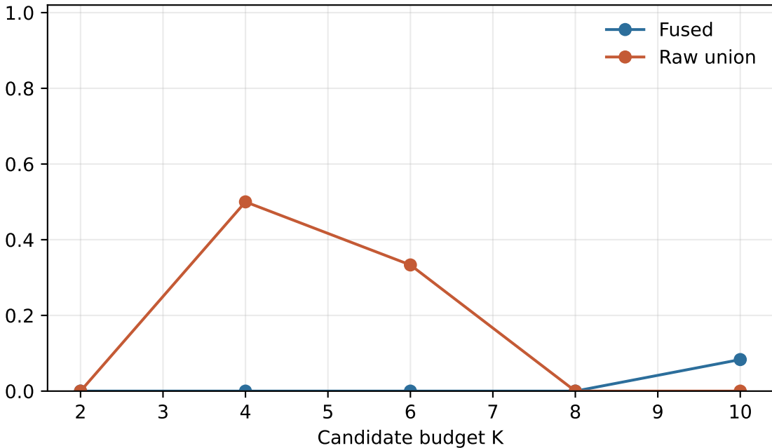
Conditional LLM choice accuracy
