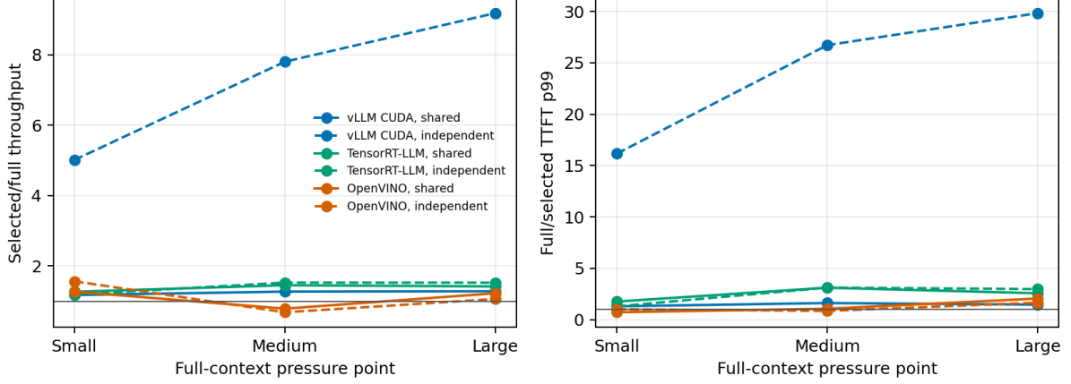
Figure 23: Within-engine throughput and TTFT-tail ratios over three context pressure points. Absolute rates are not compared across dissimilar hardware.
