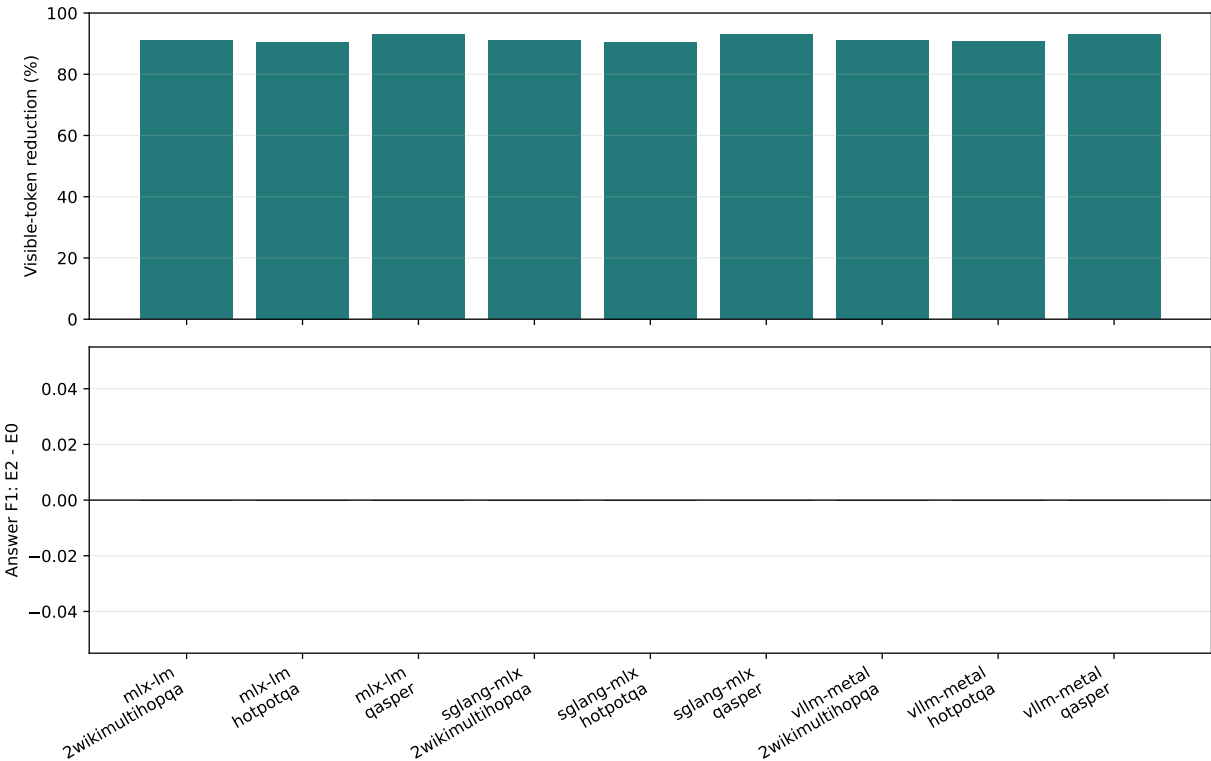
Figure 24: Holding routed evidence fixed separates visible-token reduction from semantic preservation. After restoring E0 through APC and capturing E2 from the same source prefill, all three engines retain every paired output and F1.
