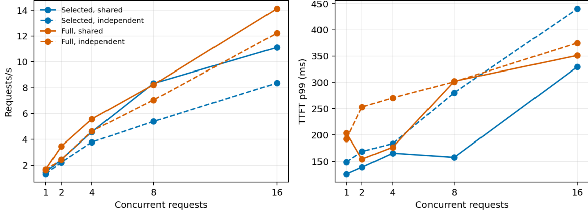
Figure 4: Expanded OpenVINO E0 throughput and TTFT tails through concurrency 16. The full-context request/s lines include wrong, shorter completions and must be read with Table 8.
