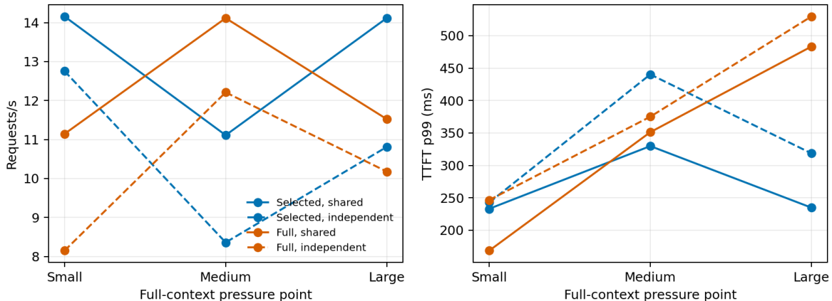
Figure 5: Peak-load throughput and TTFT tail as full visible context grows. Selected context remains fixed; solid lines share one resource and dashed lines use independent resource identities.
