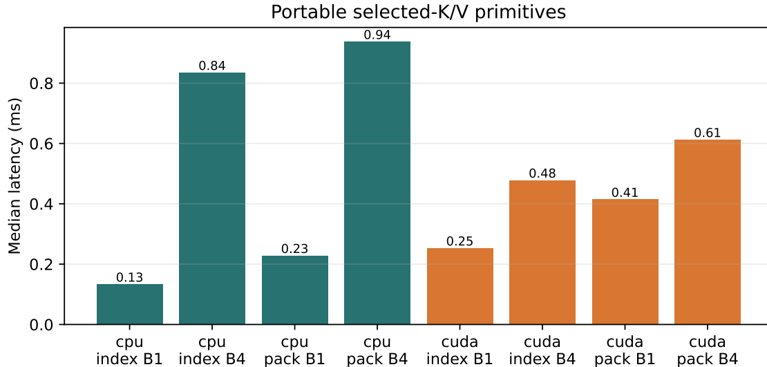
Figure 7: Portable primitive latency. This older GPU does not make small batch-one gathers faster than the CPU, but CUDA scales better at batch four.
