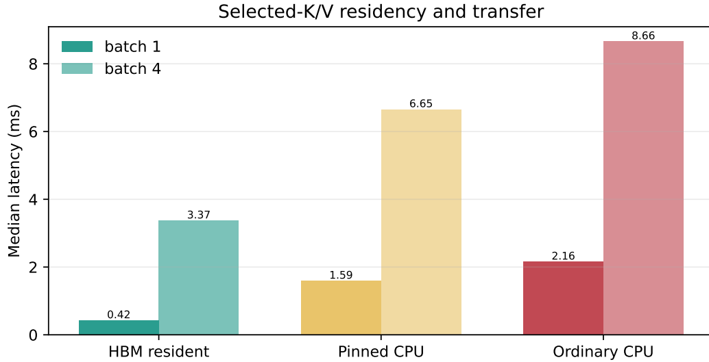
Figure 8: The same logical selection has different physical cost depending on residency. Pinned transfer helps, but does not erase the hierarchy boundary.
