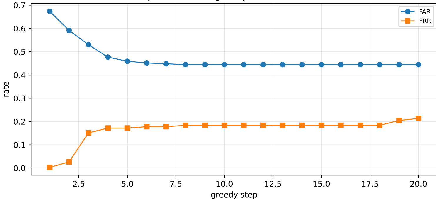
Experiment 4 — greedy forward selection
