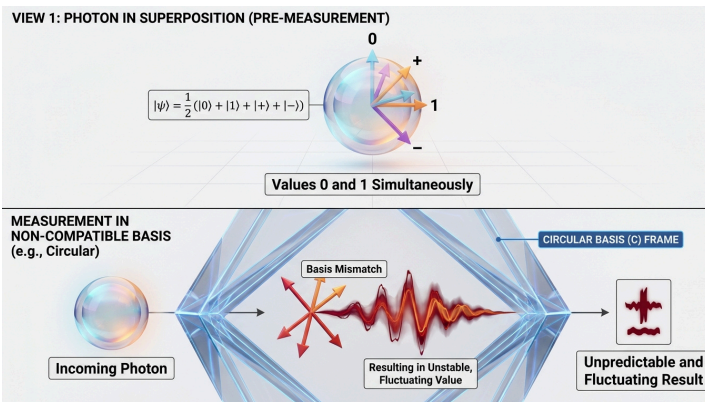
View 1: Superposition & Basis Mismatch Fluctuation (3D)
