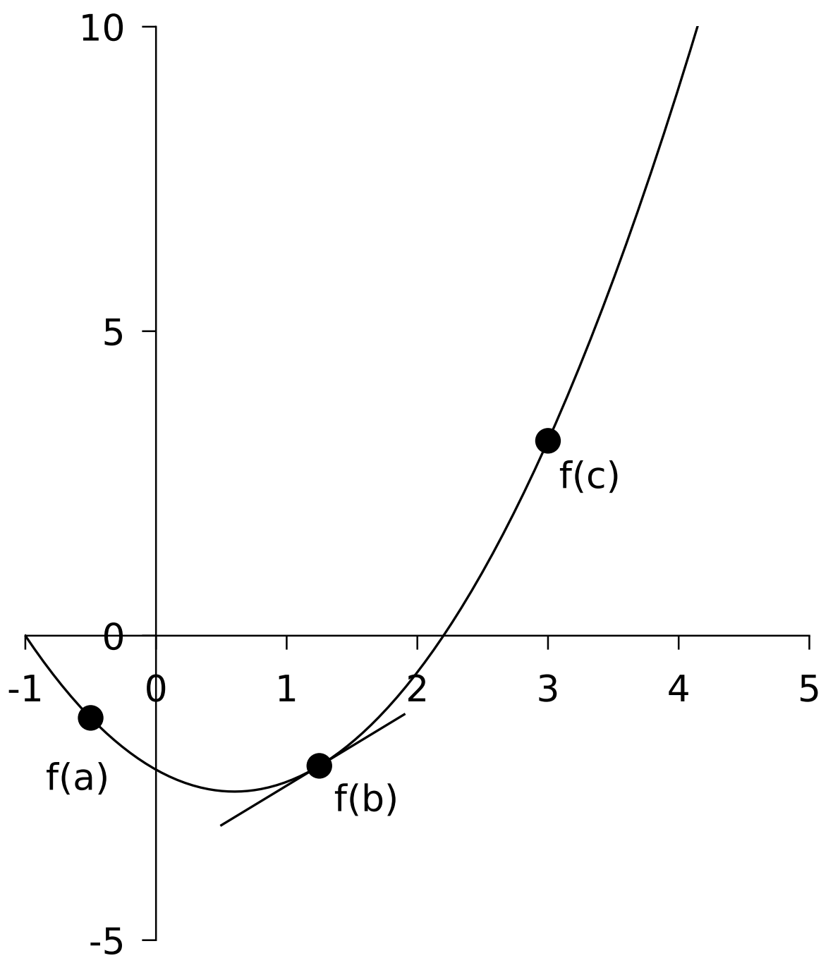
Figure 6.2: A parabola with derivative information
