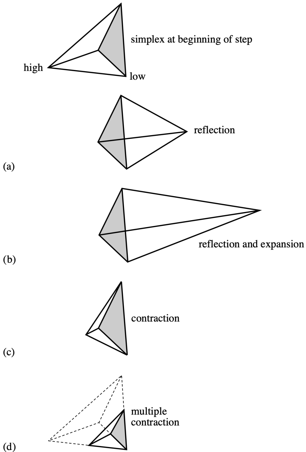
Figure 6.3: Possible outcomes for a step in the downhill simplex method. From Numerical Recipes (Press et al. 1992, fig. 10.4.1).
