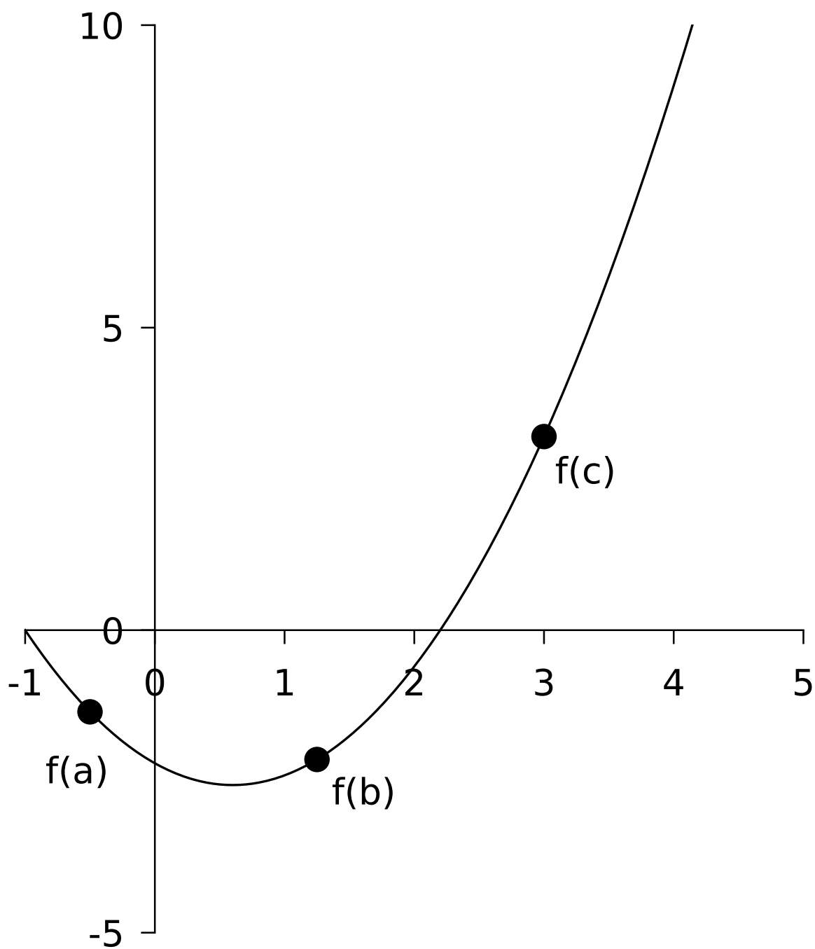
Figure 6.1: A parabola we want to minimize
