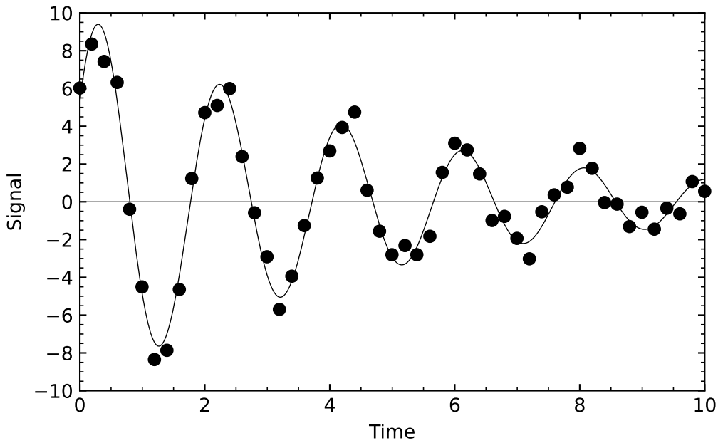
Figure 6.6: The resulting fit to the data in Figure 6.5.
