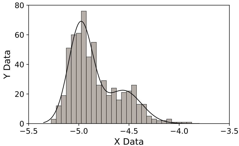
Figure 9.3: Here is the resulting fit.
