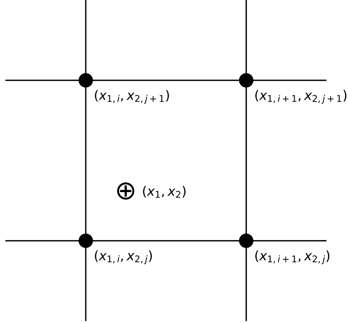
Figure 4.1: The grid cell that brackets the point (x_1, x_2) .
