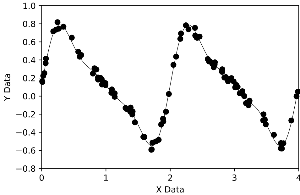
Figure 9.1: Data and resulting fit for Exercise 70.
