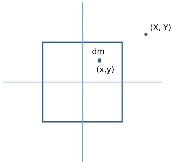
Figure 7.1: A square mass, with a mass element dm at (x, y) and the point (X, Y) outside it.
