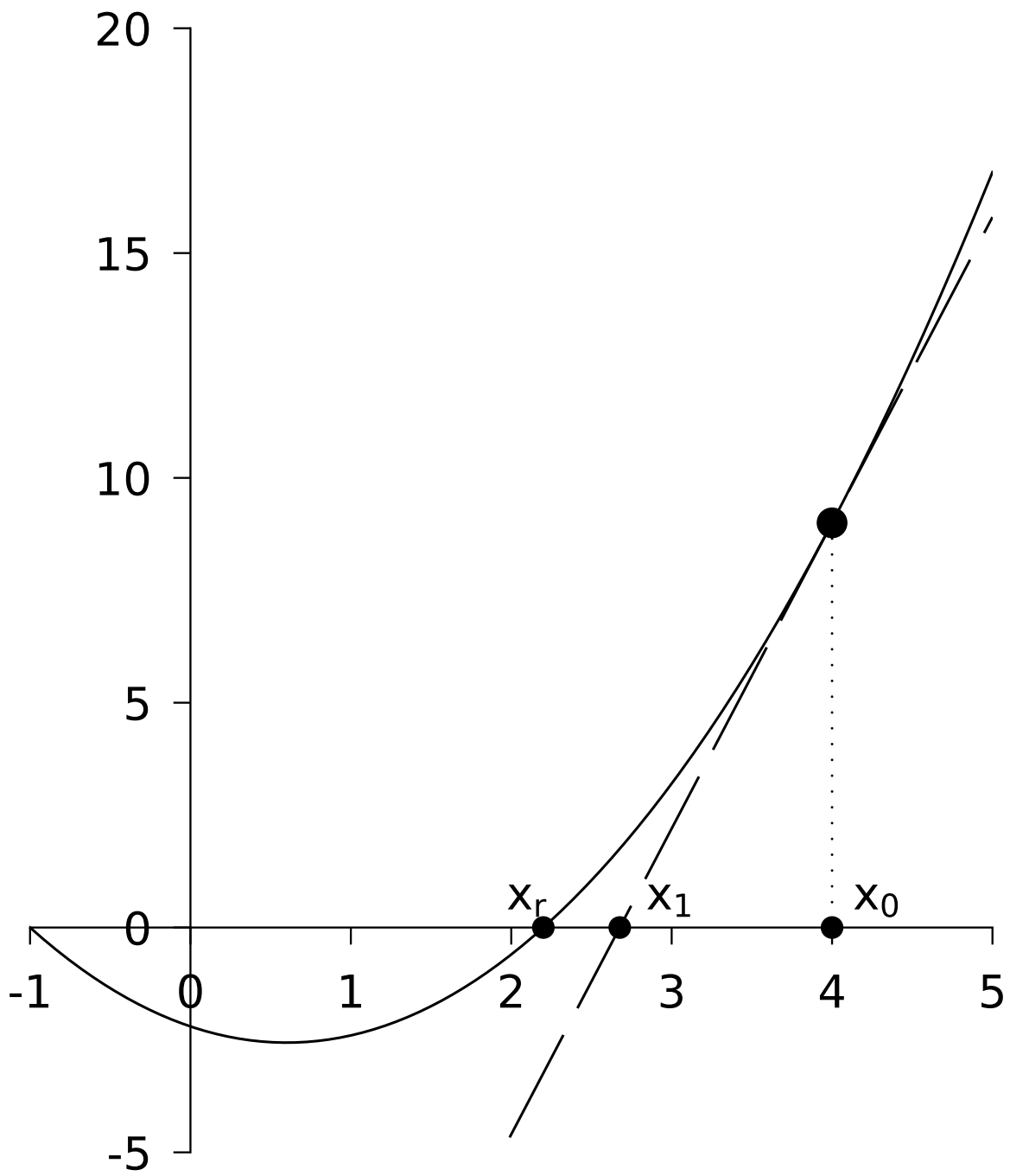
Figure 5.1: One Newton–Raphson step: the tangent at x_0 crosses zero at x_1 , closer to the root x_r .
