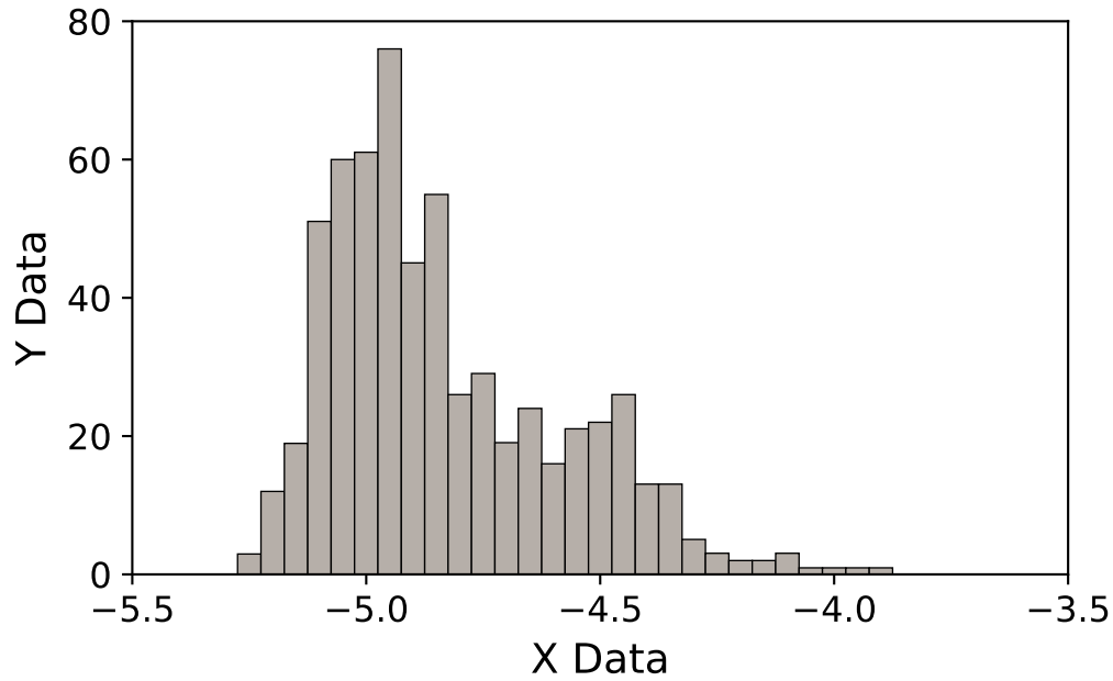
Figure 9.2: We want to fit these data with a double Gaussian.
