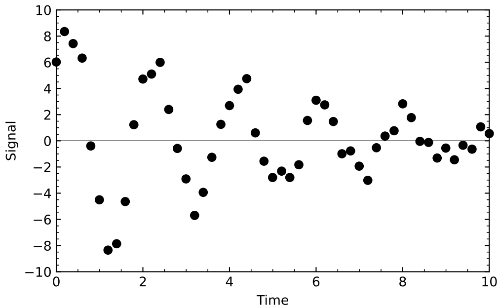
Figure 6.5: Data from an exponentially decaying oscillating system ( decay.out ).
