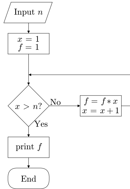
Figure 2.1: Flowchart for computing n!
