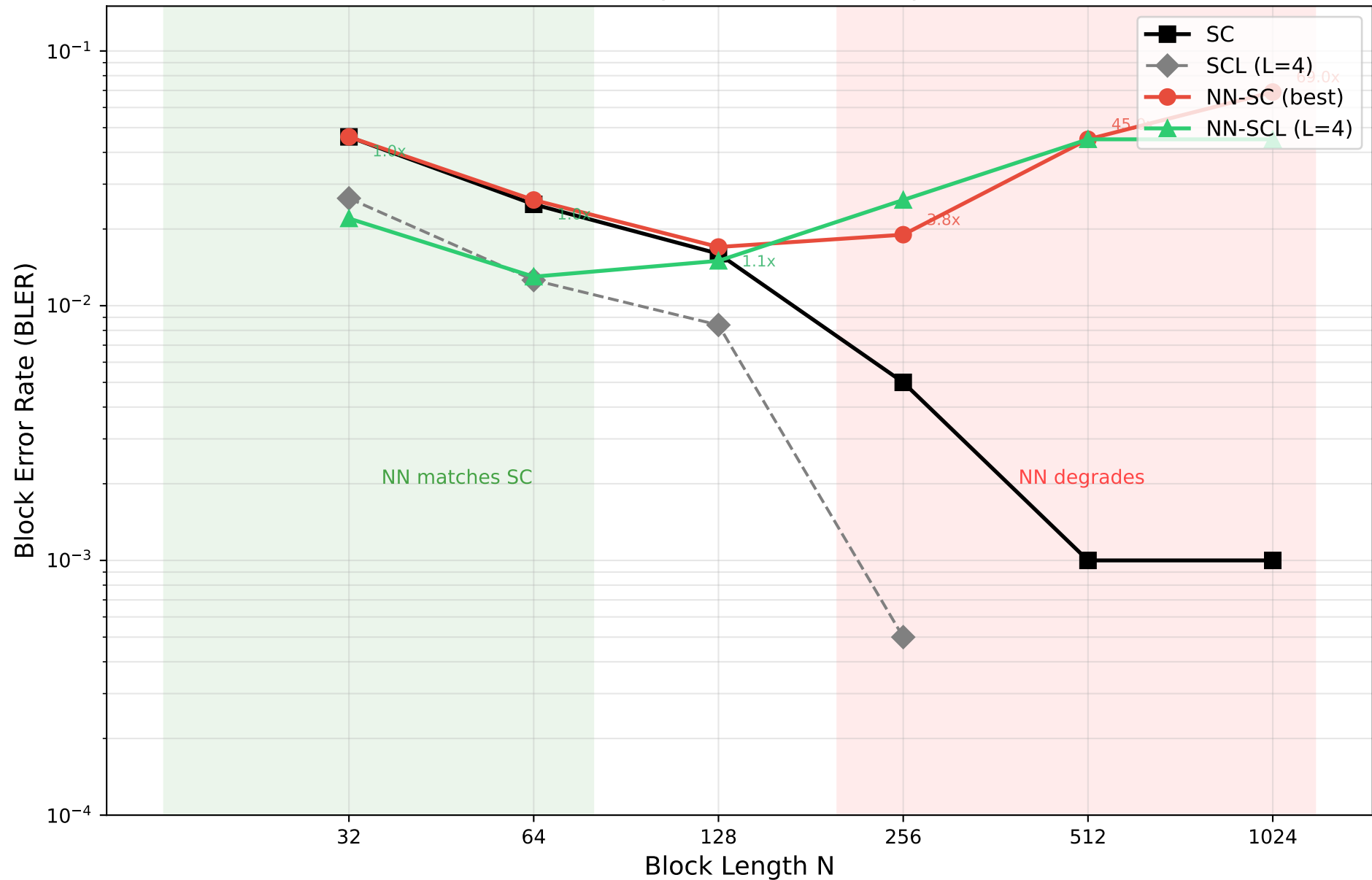
GMAC Class B (SNR=6dB, R_u \approx R_v \approx 0.48 ) Neural vs Analytical Decoders (Updated)
