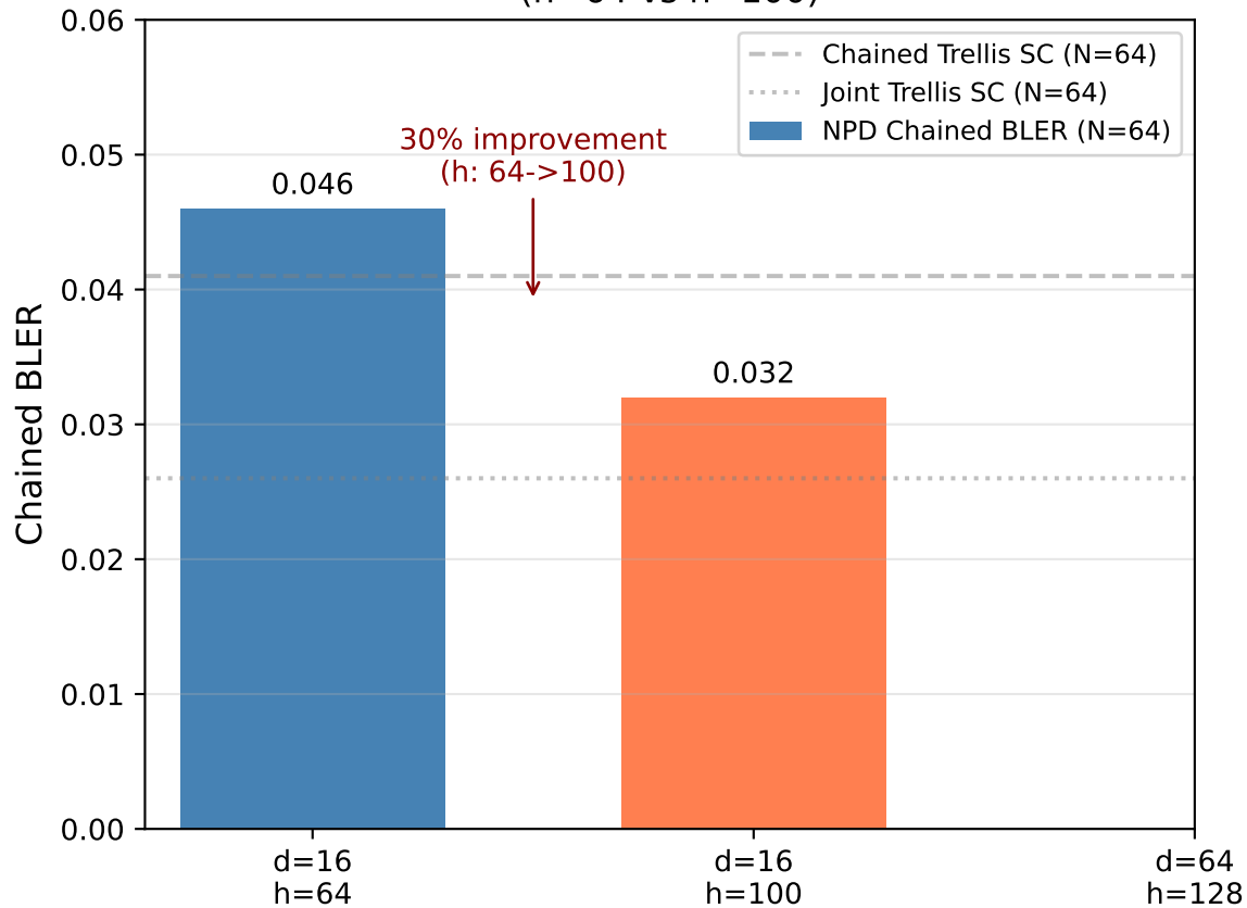
ISI-MAC N=64: Hidden Width Effect (h=64 vs h=100)
