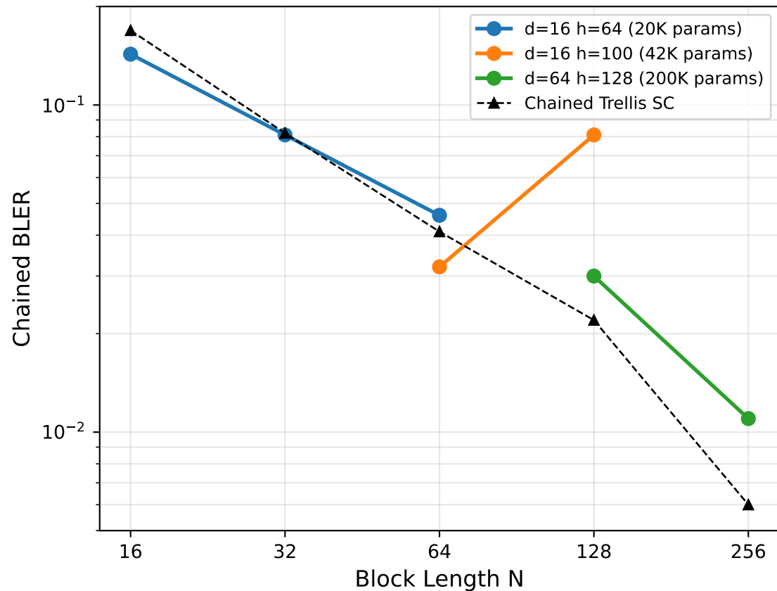
NPD Architecture Scaling (ISI-MAC, SNR=6 dB)
