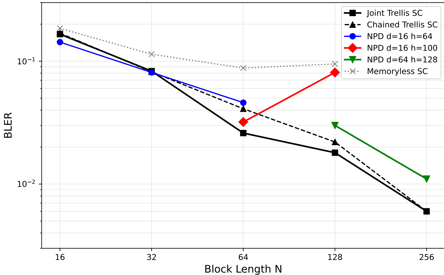
ISI-MAC Class C: NPD vs Trellis SC ( h=0.3 , SNR=6 dB, 5K-10K CW)
