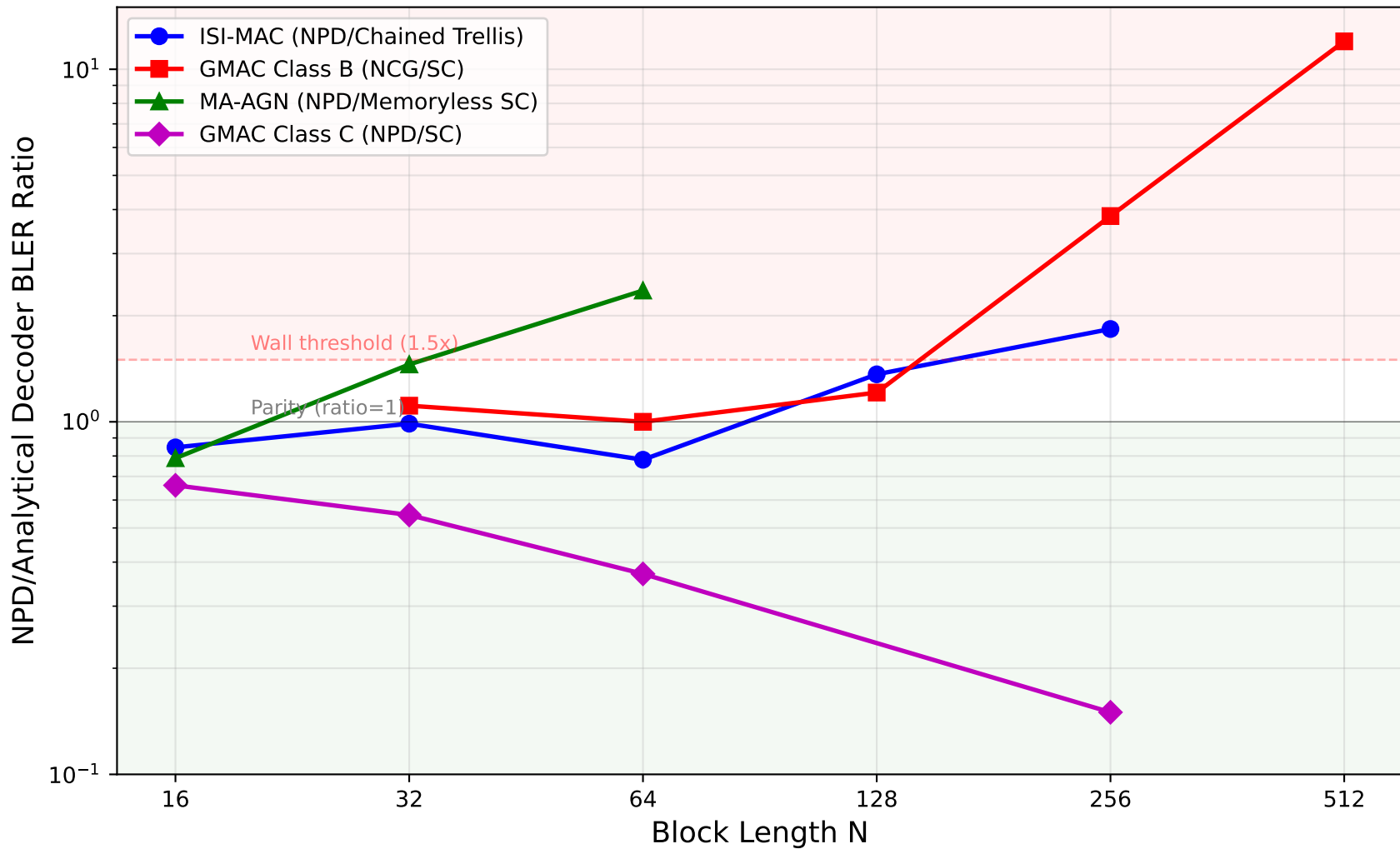
Neural Decoder Scaling: Where Walls Appear (ratio < 1 = NPD wins, ratio > 1.5 = wall)
