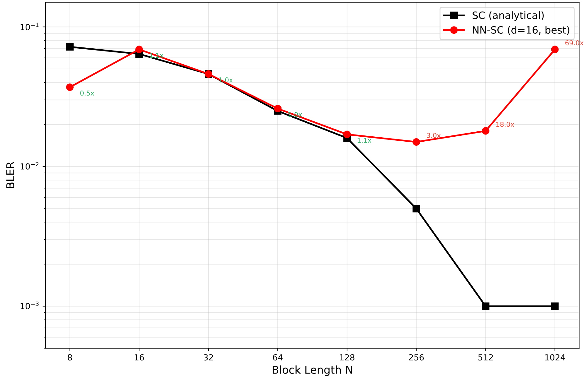
GMAC Class B (SNR=6dB) — NN vs SC R_u \approx 0.48 , R_v \approx 0.48 , Updated Apr 2
