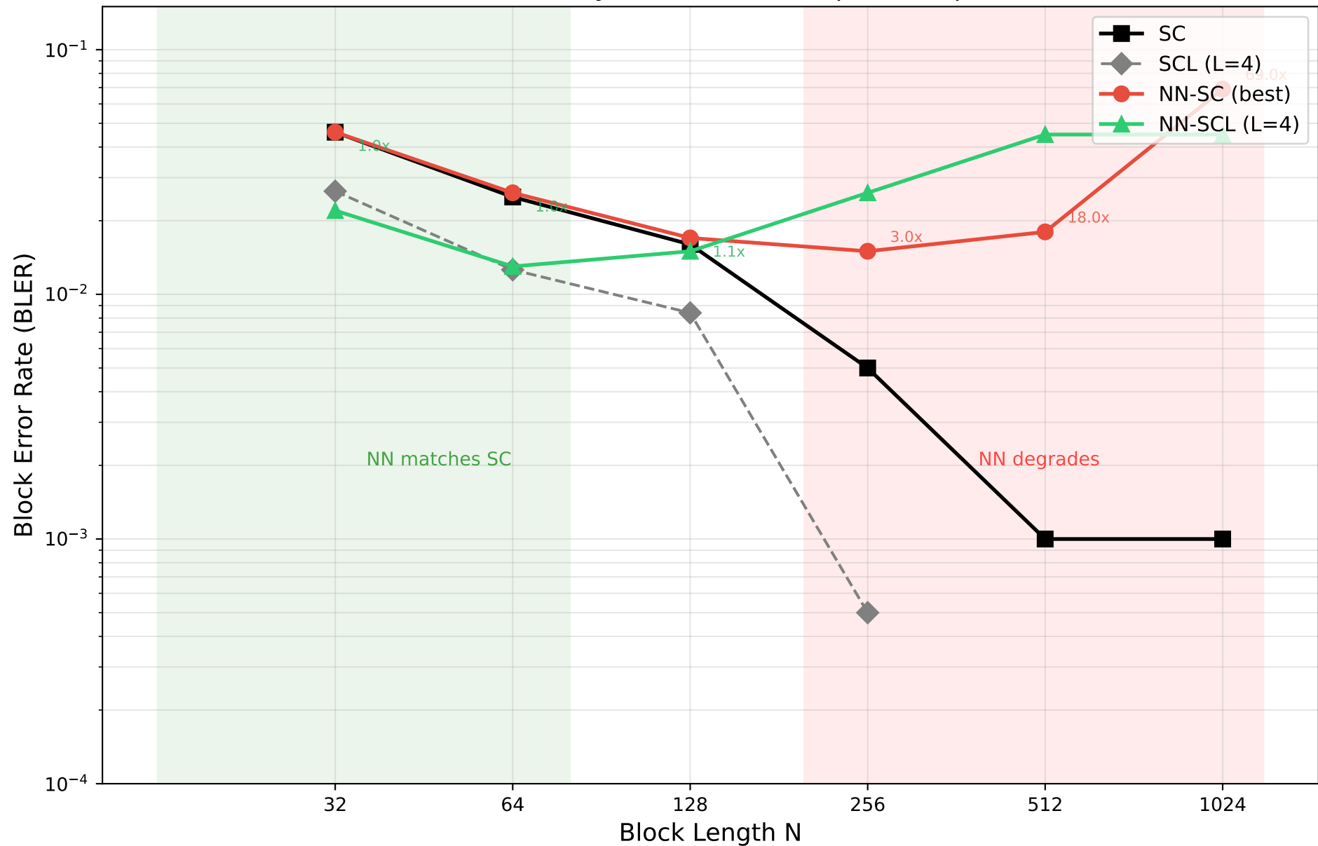
GMAC Class B (SNR=6dB, R_u \approx R_v \approx 0.48 ) Neural vs Analytical Decoders (Updated Apr 2)
