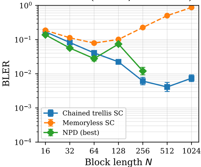
ISI-MAC ( h = 0.3 , SNR=6 dB)
