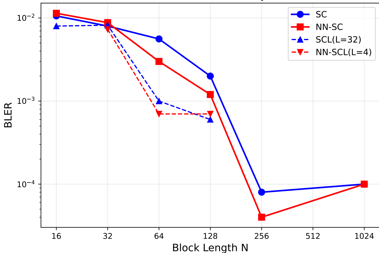
BEMAC Class B — Neural vs Analytical Decoder
