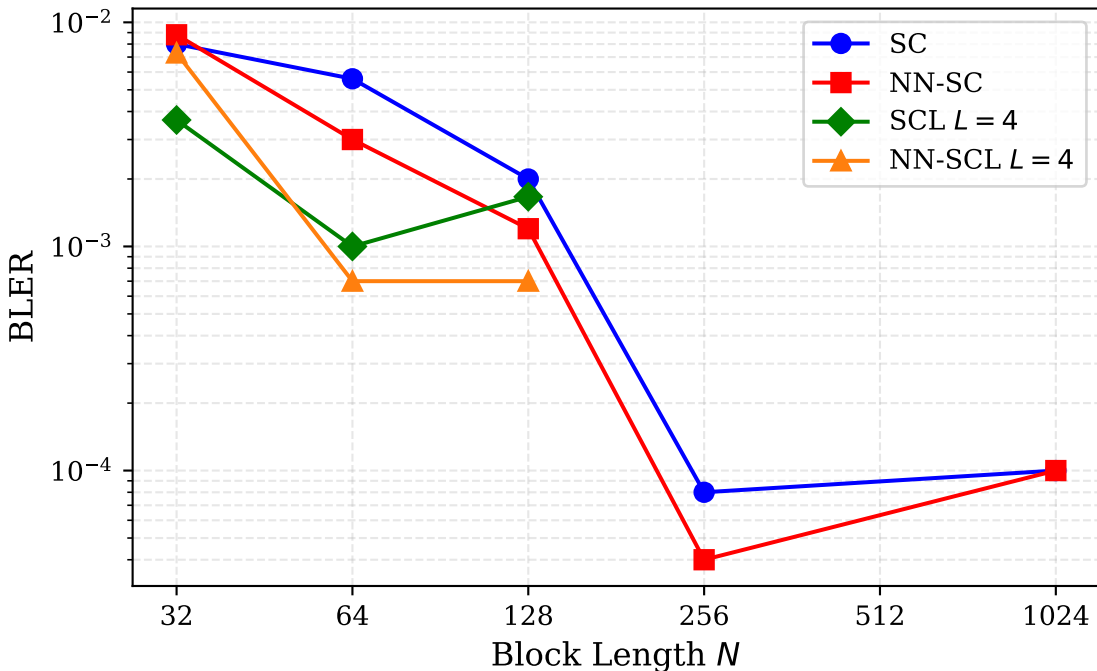
BEMAC Class B: BLER vs Block Length
