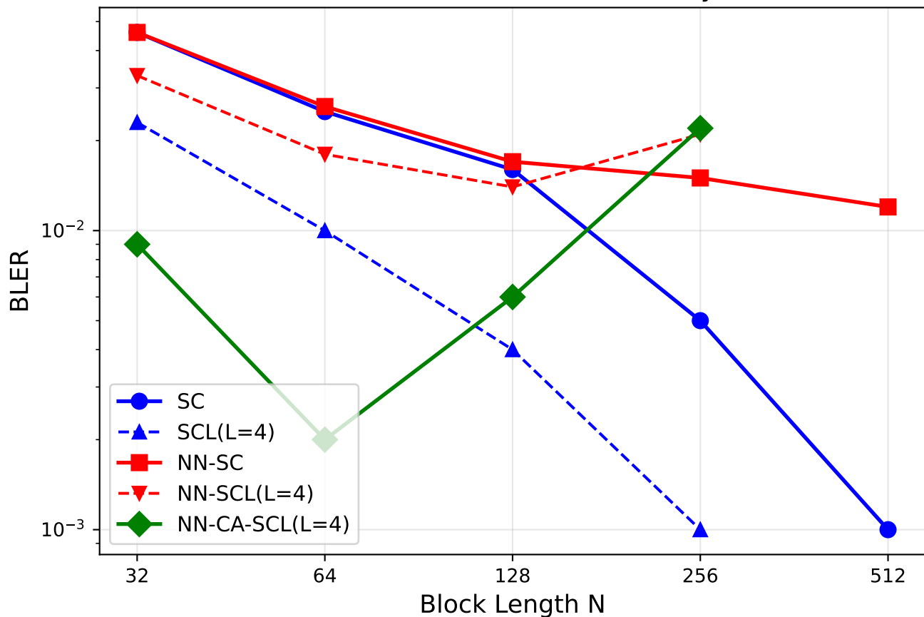
GMAC Class B, SNR=6dB — Neural vs Analytical Decoder
