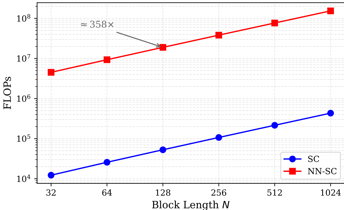
Computational Complexity: FLOPs vs Block Length
